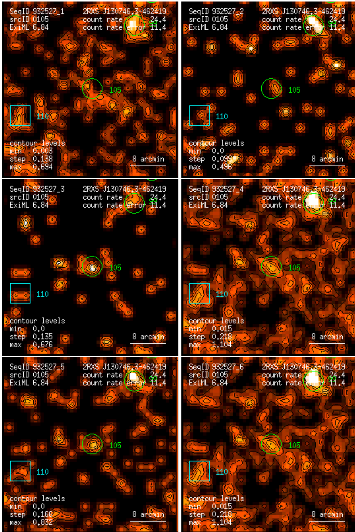
Figure 105: RASS 932527: detection 0105: band rate images, Gaussian filter: (1) PSPC channels 11 – 41, (2) 52 – 90, (3) 91 – 201, (4) 11 – 235, (5) 52 – 201, (6) 11 – 201. Broad band rates in counts/ks. Band rate contour levels in counts/ks/arcmin 2 .
