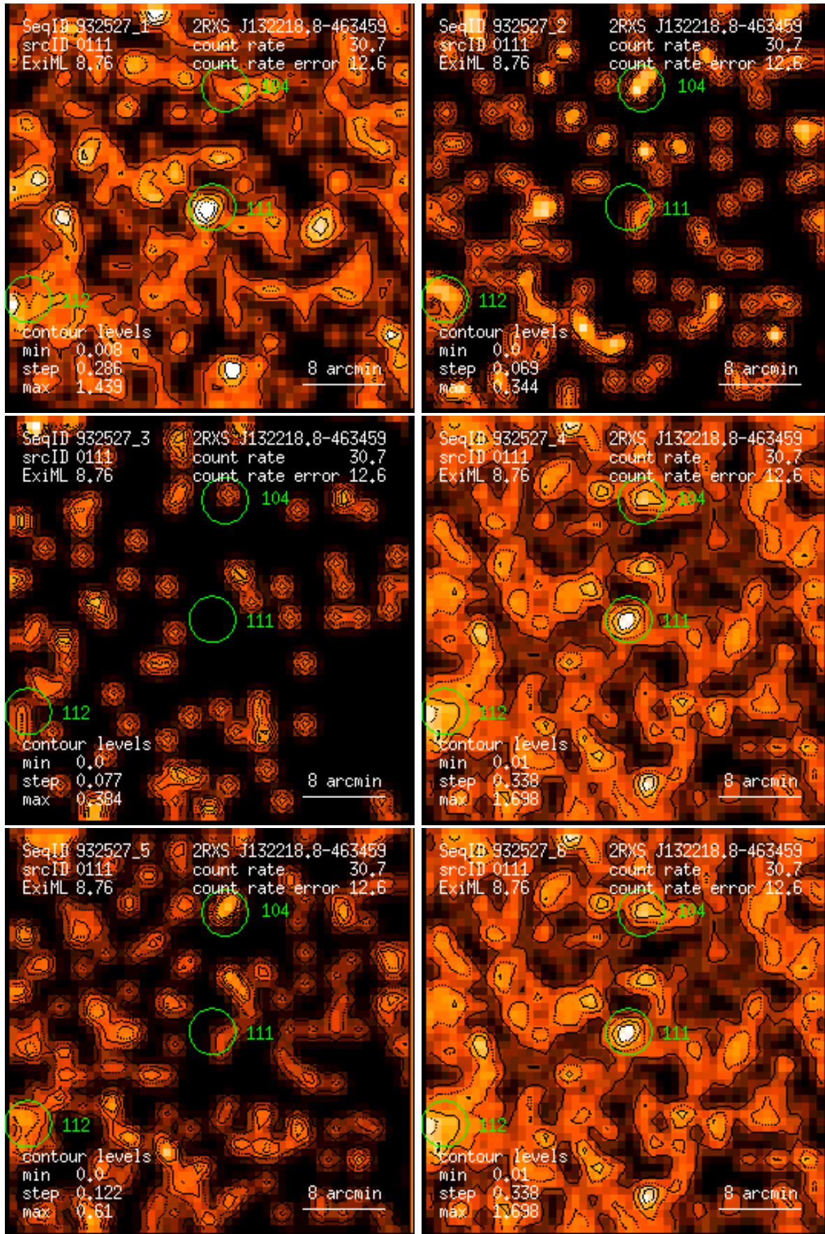
Figure 111: RASS 932527: detection 0111: band rate images, Gaussian filter: (1) PSPC channels 11 – 41, (2) 52 – 90, (3) 91 – 201, (4) 11 – 235, (5) 52 – 201, (6) 11 – 201. Broad band rates in counts/ks. Band rate contour levels in counts/ks/arcmin 2 .
