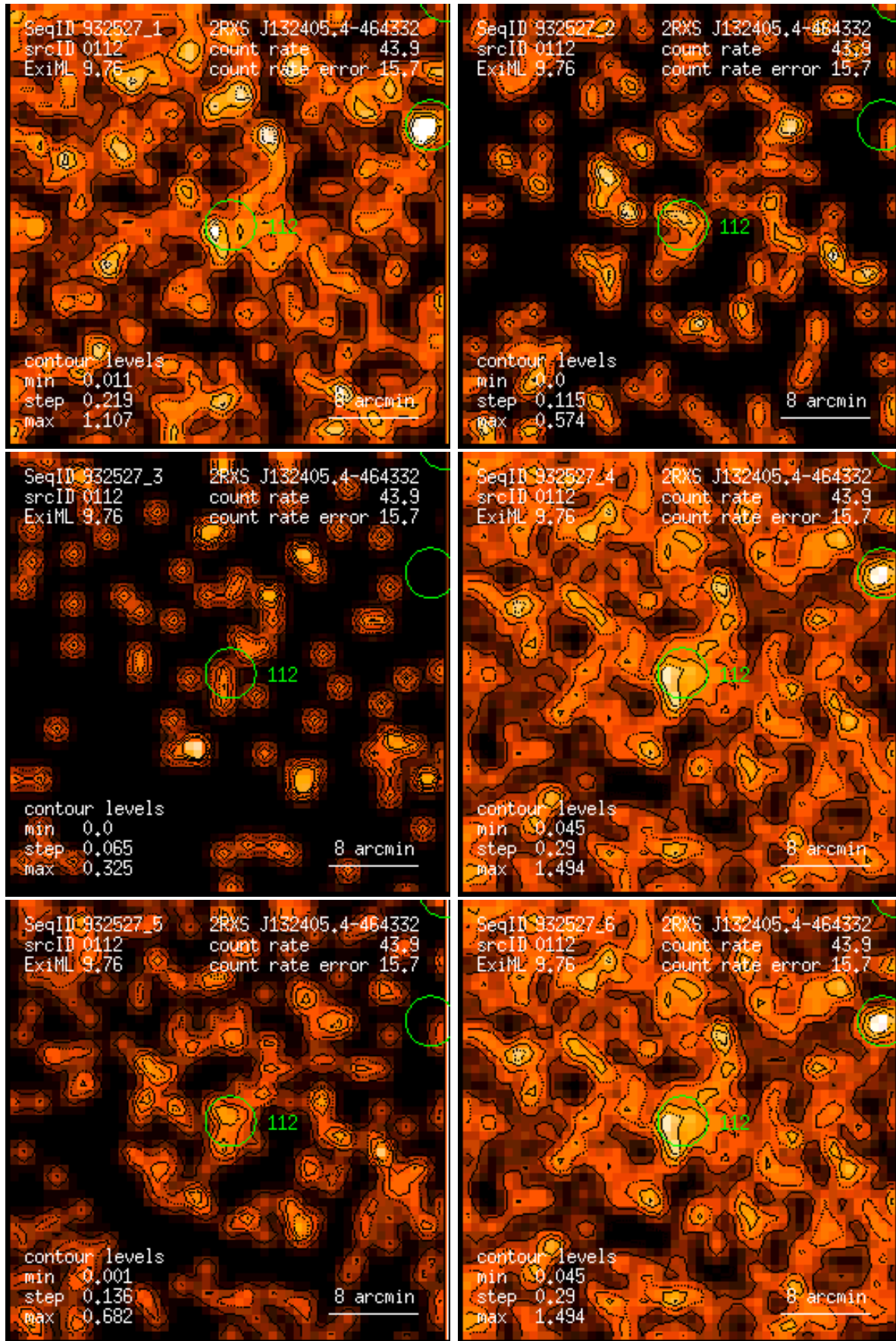
Figure 112: RASS 932527: detection 0112: band rate images, Gaussian filter: (1) PSPC channels 11 – 41, (2) 52 – 90, (3) 91 – 201, (4) 11 – 235, (5) 52 – 201, (6) 11 – 201. Broad band rates in counts/ks. Band rate contour levels in counts/ks/arcmin 2 .
