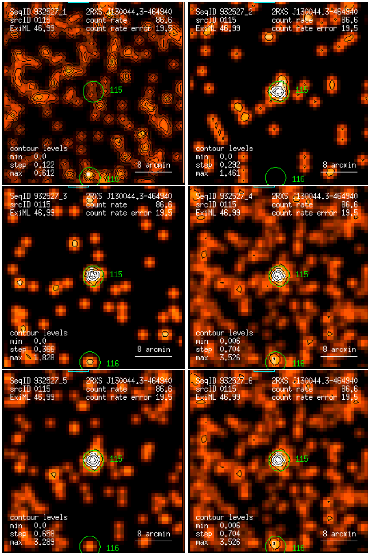
Figure 115: RASS 932527: detection 0115: band rate images, Gaussian filter: (1) PSPC channels 11 – 41, (2) 52 – 90, (3) 91 – 201, (4) 11 – 235, (5) 52 – 201, (6) 11 – 201. Broad band rates in counts/ks. Band rate contour levels in counts/ks/arcmin 2 .
