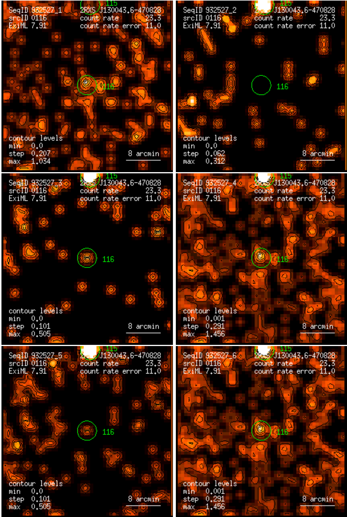
Figure 116: RASS 932527: detection 0116: band rate images, Gaussian filter: (1) PSPC channels 11 – 41, (2) 52 – 90, (3) 91 – 201, (4) 11 – 235, (5) 52 – 201, (6) 11 – 201. Broad band rates in counts/ks. Band rate contour levels in counts/ks/arcmin 2 .
