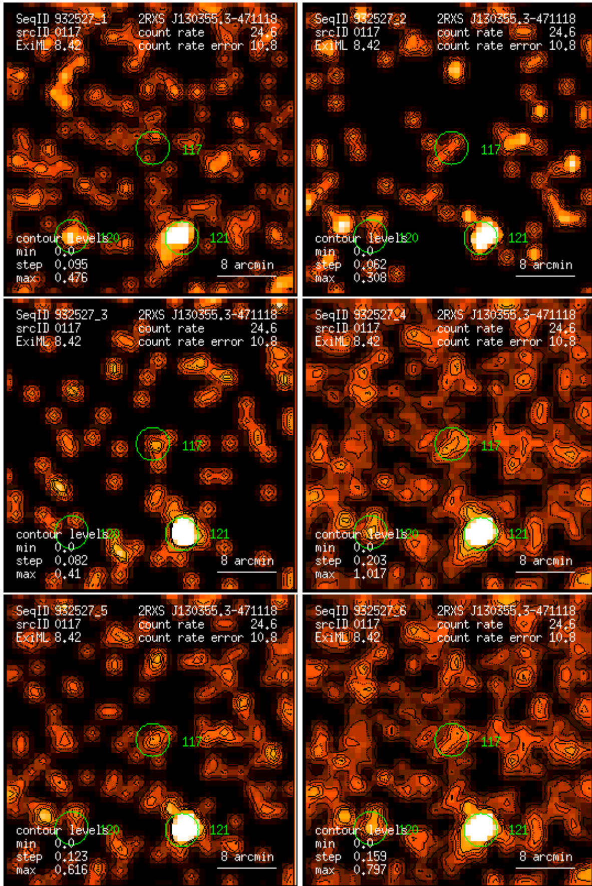
Figure 117: RASS 932527: detection 0117: band rate images, Gaussian filter: (1) PSPC channels 11 – 41, (2) 52 – 90, (3) 91 – 201, (4) 11 – 235, (5) 52 – 201, (6) 11 – 201. Broad band rates in counts/ks. Band rate contour levels in counts/ks/arcmin 2 .
