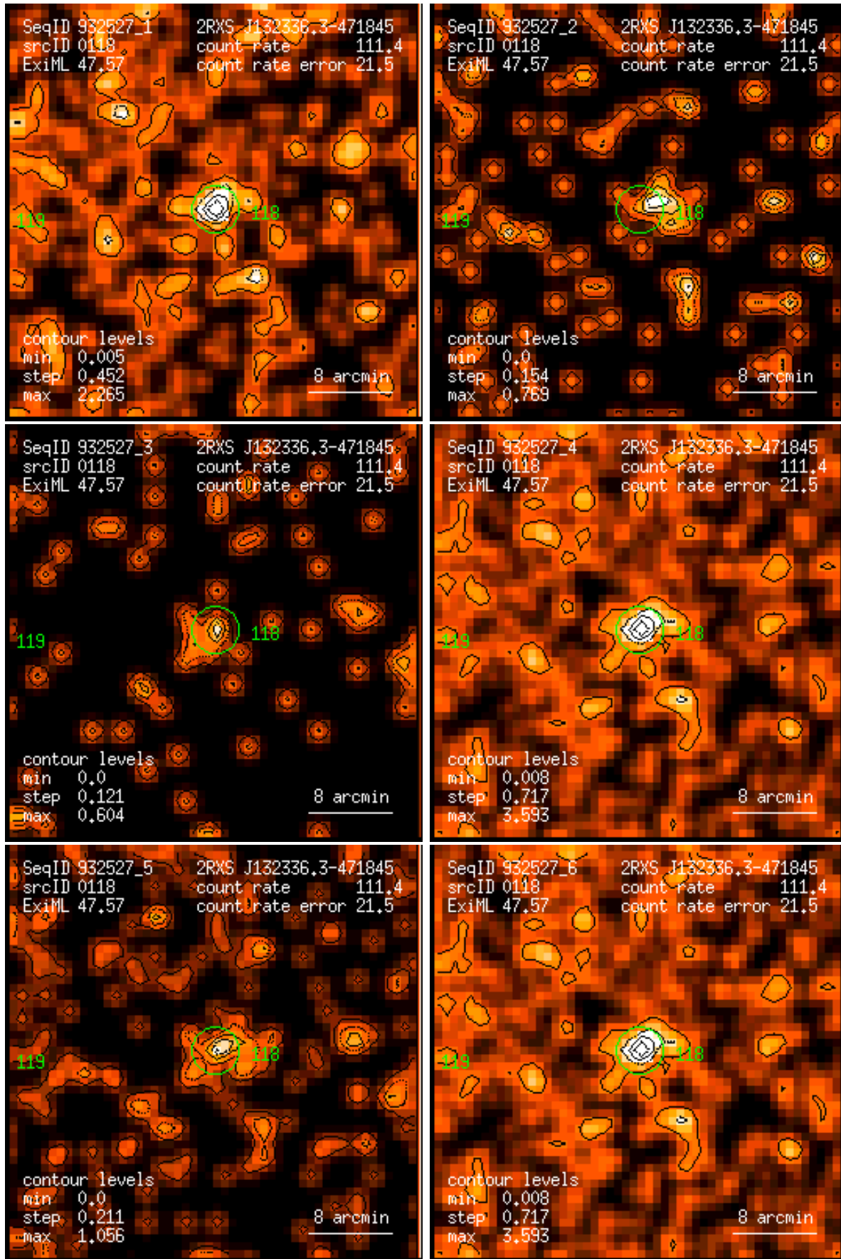
Figure 118: RASS 932527: detection 0118: band rate images, Gaussian filter: (1) PSPC channels 11 – 41, (2) 52 – 90, (3) 91 – 201, (4) 11 – 235, (5) 52 – 201, (6) 11 – 201. Broad band rates in counts/ks. Band rate contour levels in counts/ks/arcmin 2 .
