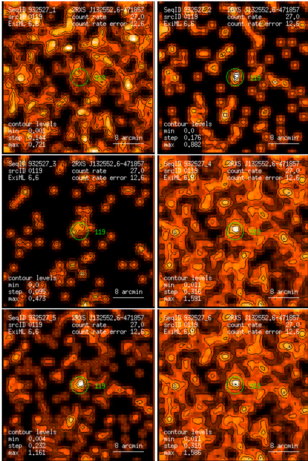
Figure 119: RASS 932527: detection 0119: band rate images, Gaussian filter: (1) PSPC channels 11 – 41, (2) 52 – 90, (3) 91 – 201, (4) 11 – 235, (5) 52 – 201, (6) 11 – 201. Broad band rates in counts/ks. Band rate contour levels in counts/ks/arcmin 2 .
