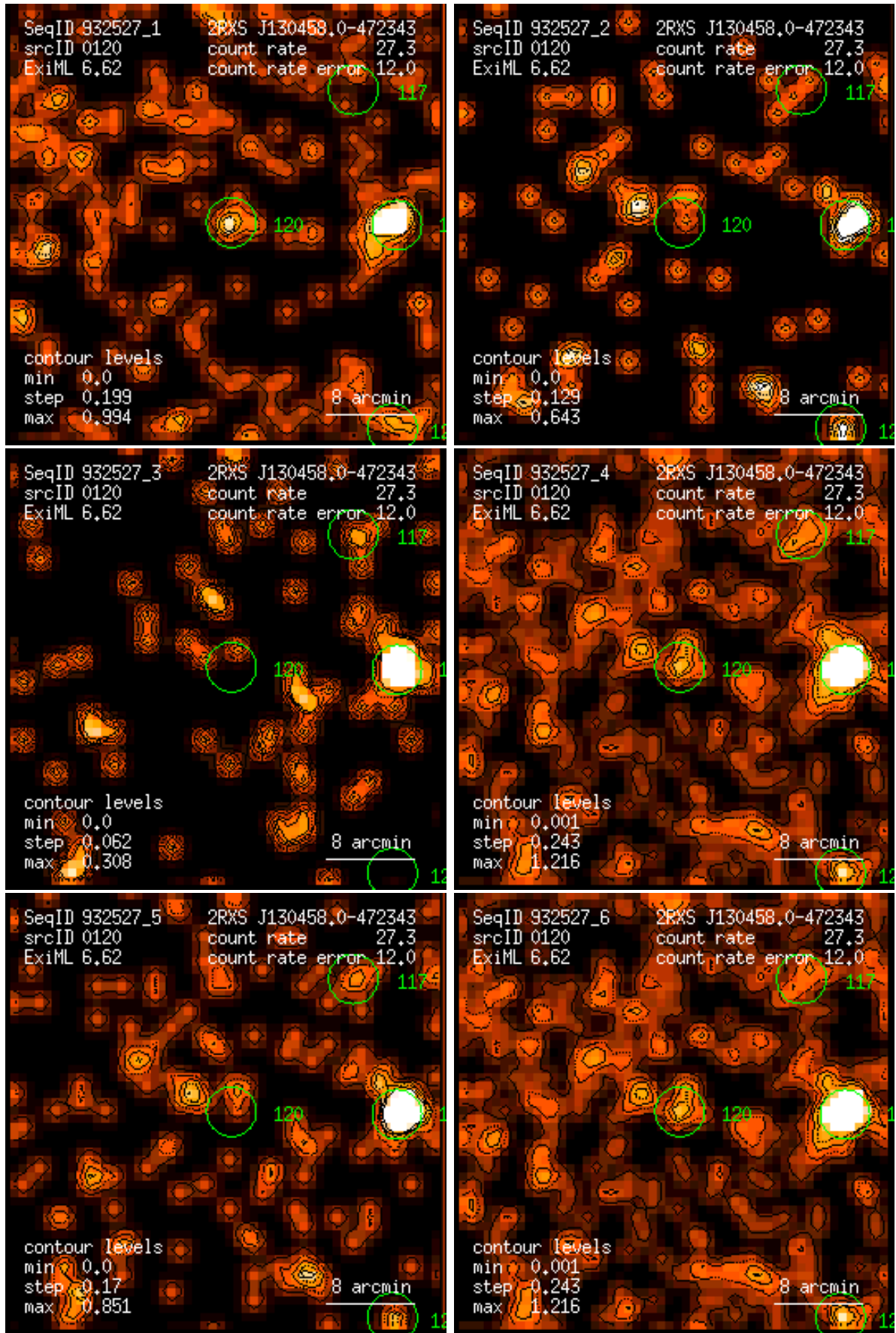
Figure 120: RASS 932527: detection 0120: band rate images, Gaussian filter: (1) PSPC channels 11 – 41, (2) 52 – 90, (3) 91 – 201, (4) 11 – 235, (5) 52 – 201, (6) 11 – 201. Broad band rates in counts/ks. Band rate contour levels in counts/ks/arcmin 2 .
