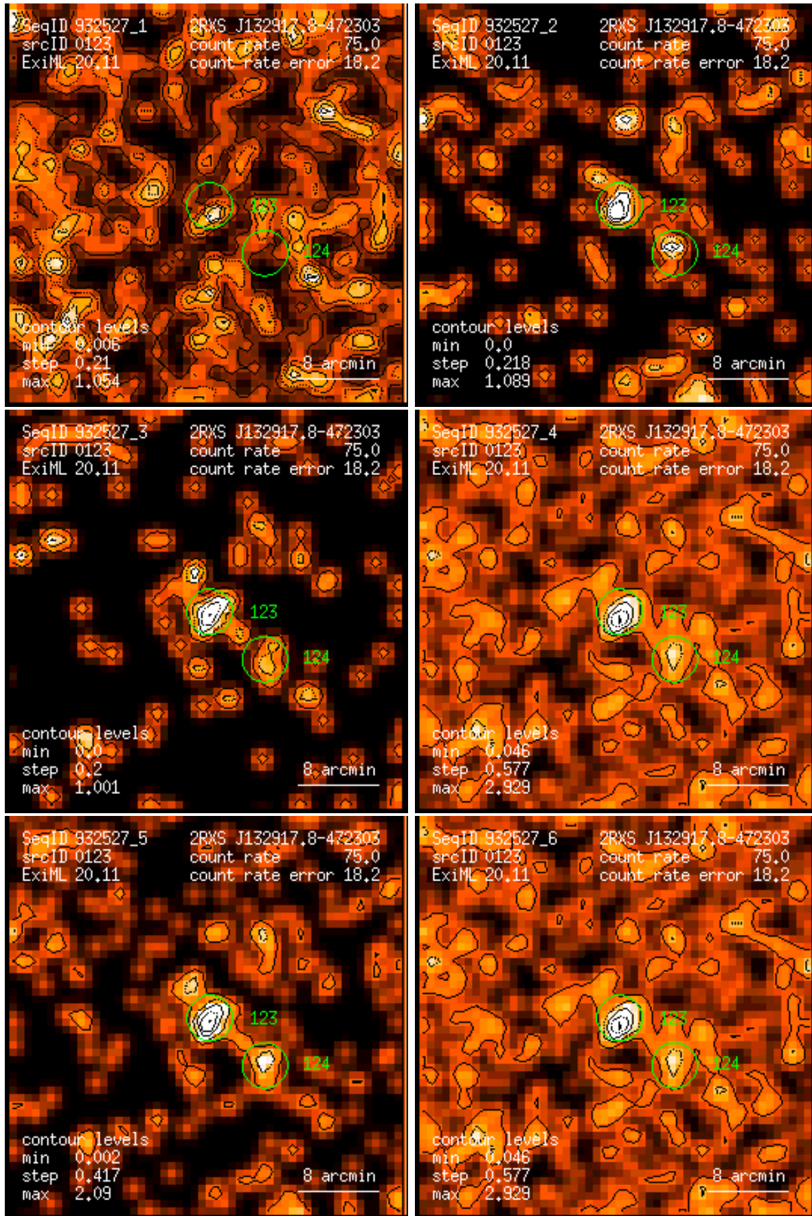
Figure 123: RASS 932527: detection 0123: band rate images, Gaussian filter: (1) PSPC channels 11 – 41, (2) 52 – 90, (3) 91 – 201, (4) 11 – 235, (5) 52 – 201, (6) 11 – 201. Broad band rates in counts/ks. Band rate contour levels in counts/ks/arcmin 2 .
