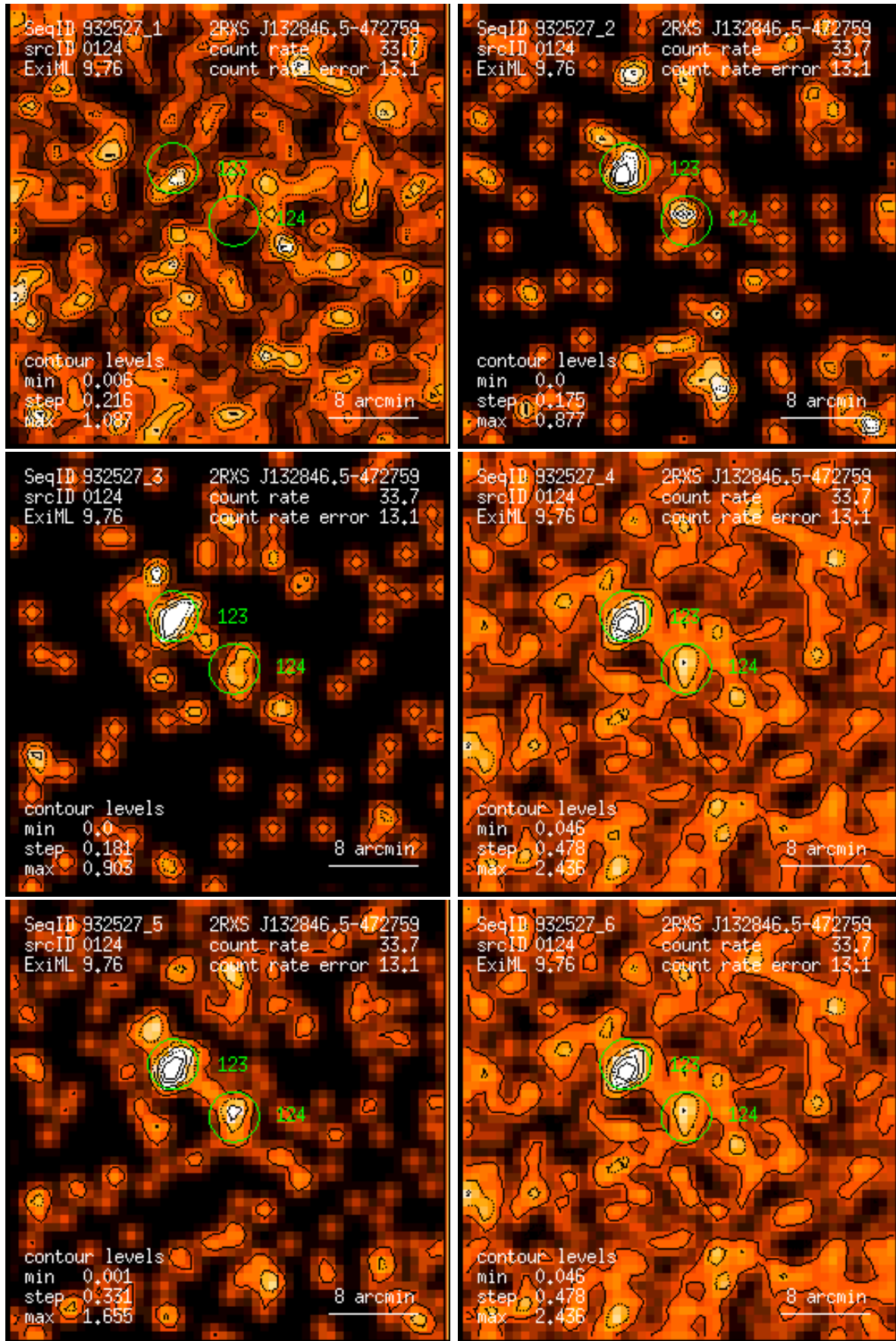
Figure 124: RASS 932527: detection 0124: band rate images, Gaussian filter: (1) PSPC channels 11 – 41, (2) 52 – 90, (3) 91 – 201, (4) 11 – 235, (5) 52 – 201, (6) 11 – 201. Broad band rates in counts/ks. Band rate contour levels in counts/ks/arcmin 2 .
