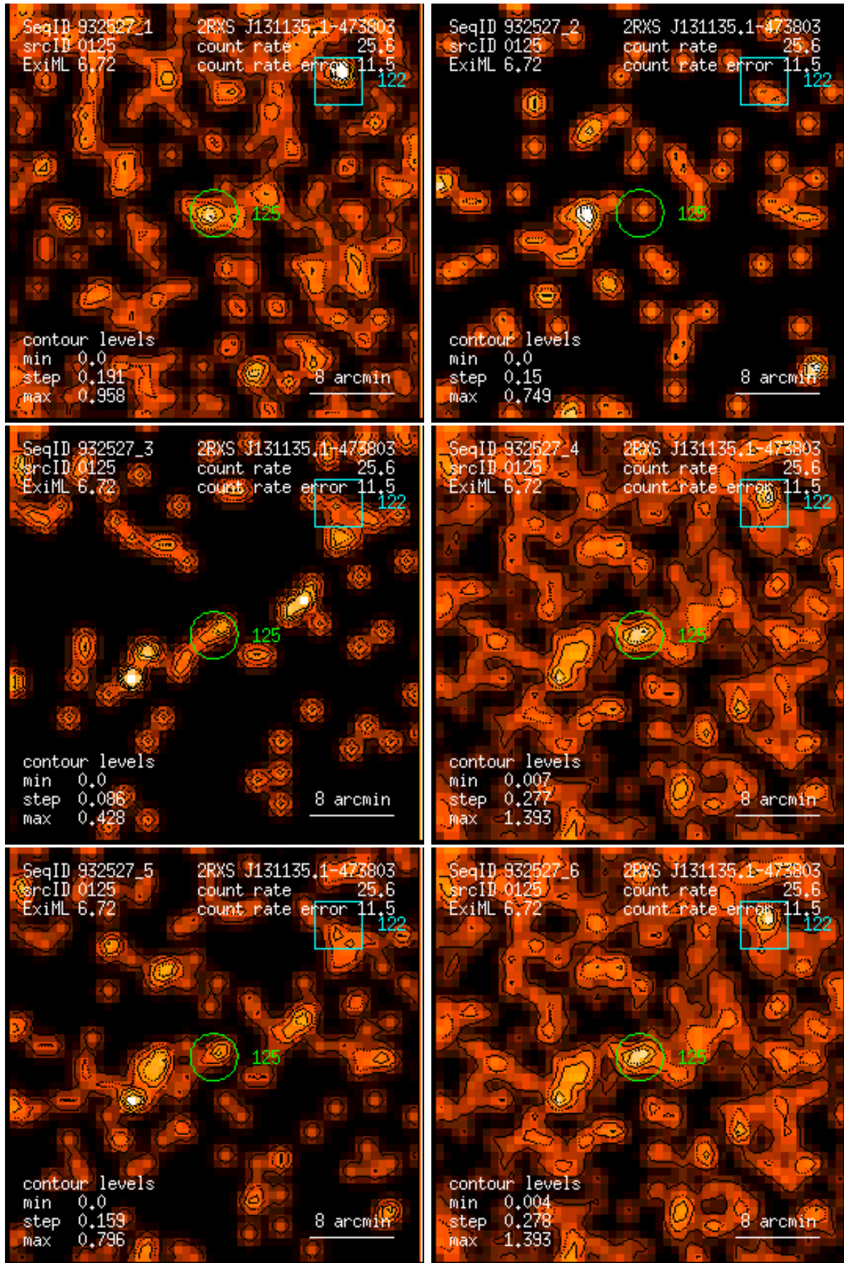
Figure 125: RASS 932527: detection 0125: band rate images, Gaussian filter: (1) PSPC channels 11 – 41, (2) 52 – 90, (3) 91 – 201, (4) 11 – 235, (5) 52 – 201, (6) 11 – 201. Broad band rates in counts/ks. Band rate contour levels in counts/ks/arcmin 2 .
