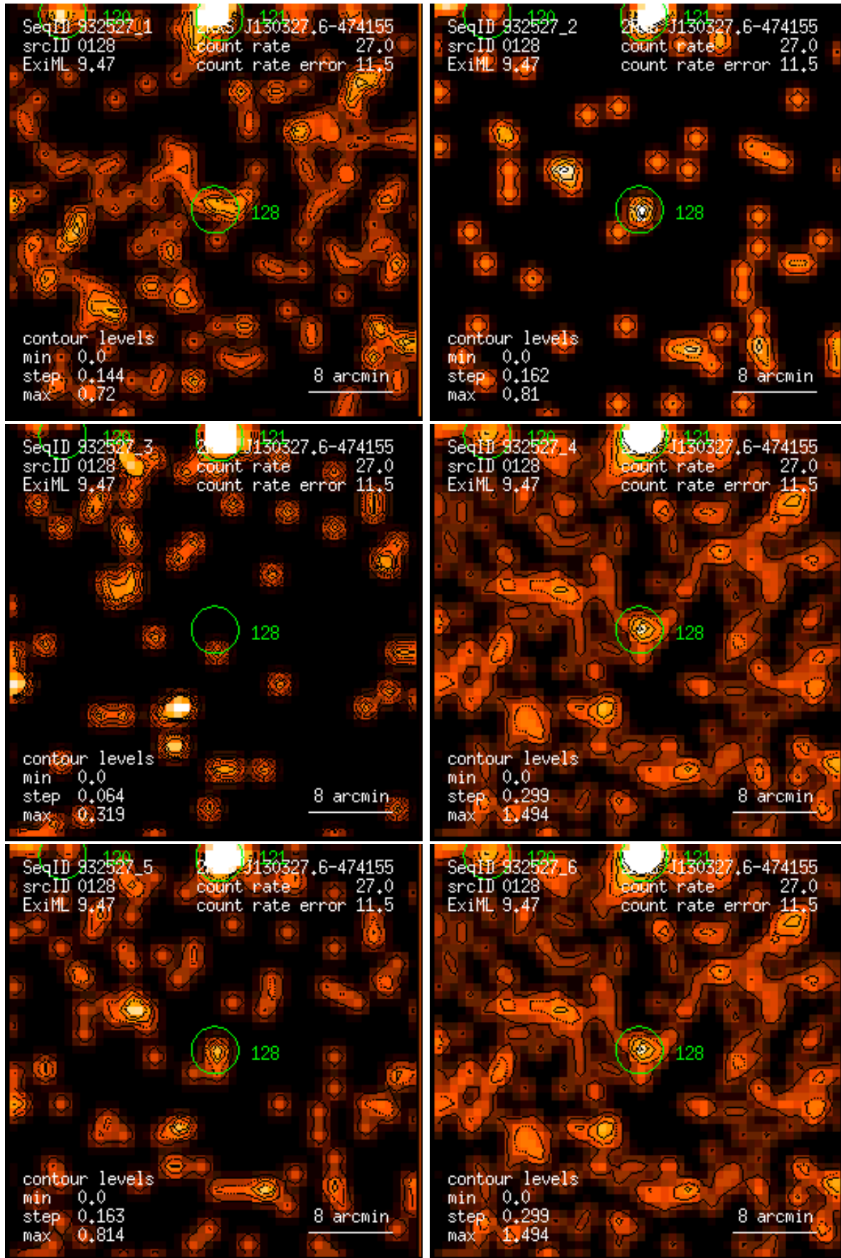
Figure 128: RASS 932527: detection 0128: band rate images, Gaussian filter: (1) PSPC channels 11 – 41, (2) 52 – 90, (3) 91 – 201, (4) 11 – 235, (5) 52 – 201, (6) 11 – 201. Broad band rates in counts/ks. Band rate contour levels in counts/ks/arcmin 2 .
