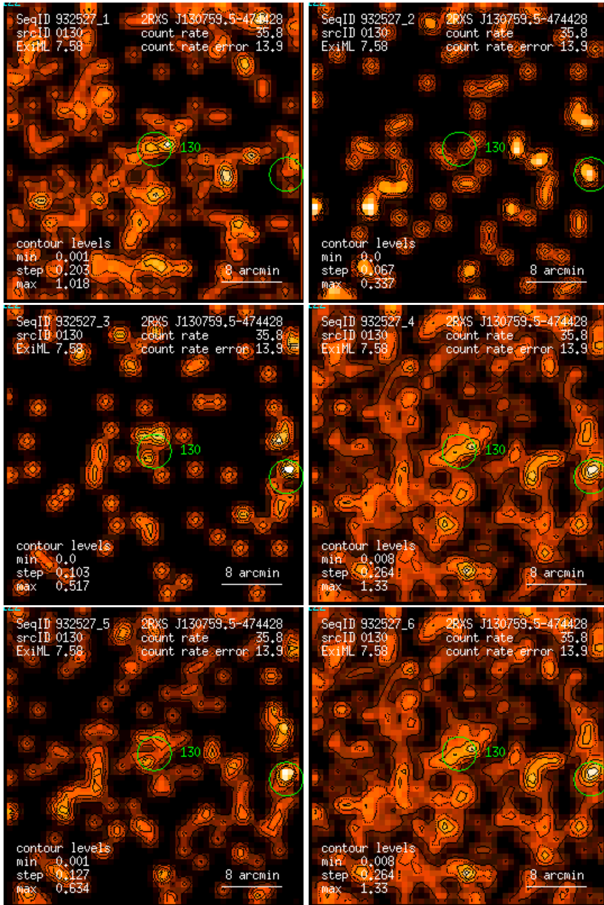
Figure 130: RASS 932527: detection 0130: band rate images, Gaussian filter: (1) PSPC channels 11 – 41, (2) 52 – 90, (3) 91 – 201, (4) 11 – 235, (5) 52 – 201, (6) 11 – 201. Broad band rates in counts/ks. Band rate contour levels in counts/ks/arcmin 2 .
