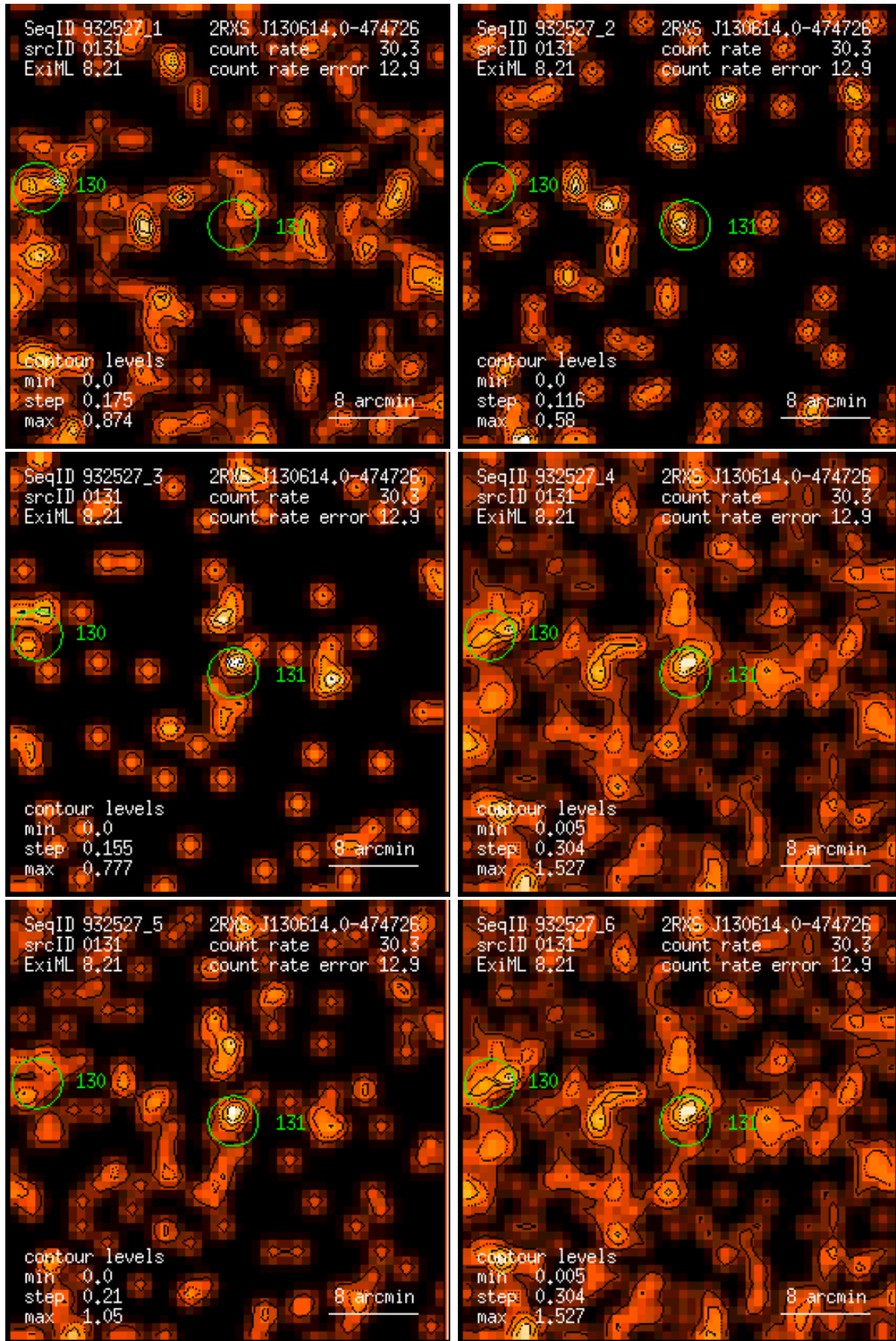
Figure 131: RASS 932527: detection 0131: band rate images, Gaussian filter: (1) PSPC channels 11 – 41, (2) 52 – 90, (3) 91 – 201, (4) 11 – 235, (5) 52 – 201, (6) 11 – 201. Broad band rates in counts/ks. Band rate contour levels in counts/ks/arcmin 2 .
