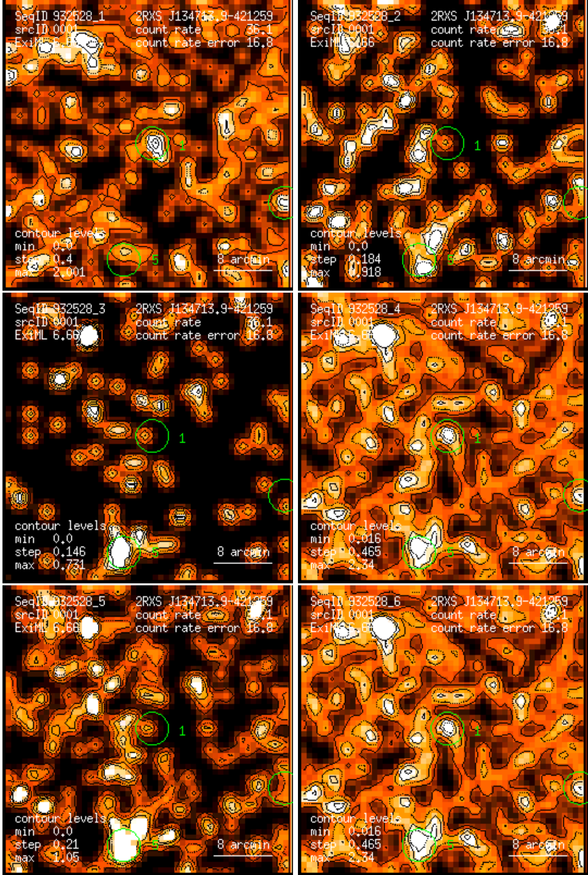
Figure 1: RASS 932528: detection 0001: band rate images, Gaussian filter: (1) PSPC channels 11 – 41, (2) 52 – 90, (3) 91 – 201, (4) 11 – 235, (5) 52 – 201, (6) 11 – 201. Broad band rates in counts/ks. Band rate contour levels in counts/ks/arcmin 2 .
