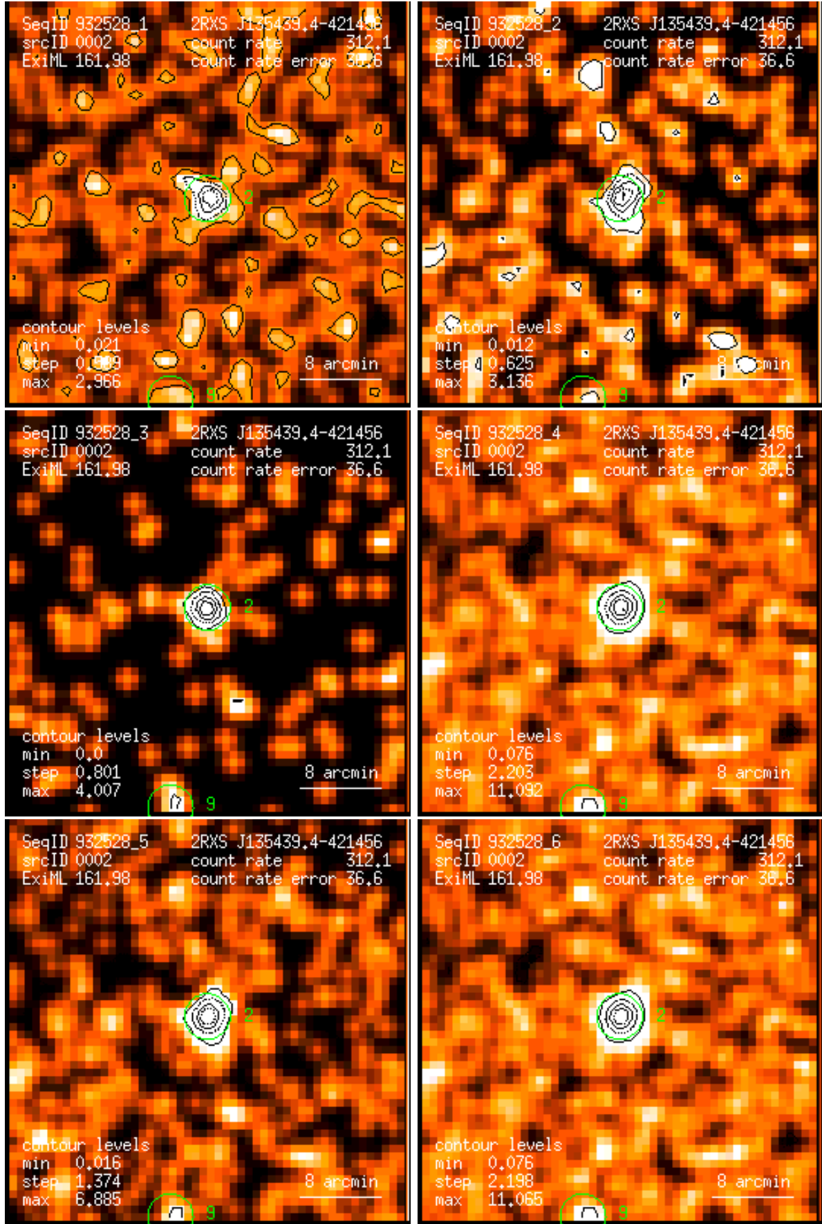
Figure 2: RASS 932528: detection 0002: band rate images, Gaussian filter: (1) PSPC channels 11 – 41, (2) 52 – 90, (3) 91 – 201, (4) 11 – 235, (5) 52 – 201, (6) 11 – 201. Broad band rates in counts/ks. Band rate contour levels in counts/ks/arcmin 2 .
