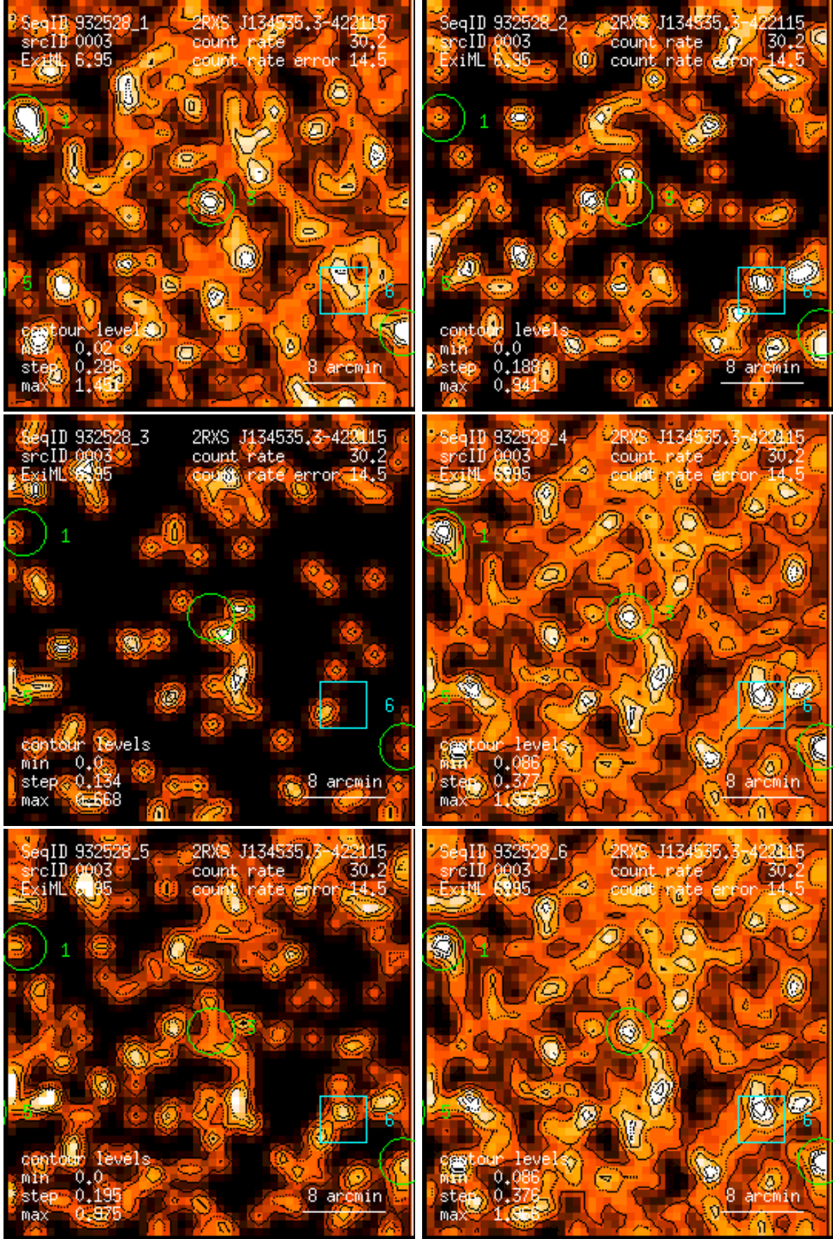
Figure 3: RASS 932528: detection 0003: band rate images, Gaussian filter: (1) PSPC channels 11 – 41, (2) 52 – 90, (3) 91 – 201, (4) 11 – 235, (5) 52 – 201, (6) 11 – 201. Broad band rates in counts/ks. Band rate contour levels in counts/ks/arcmin 2 .
