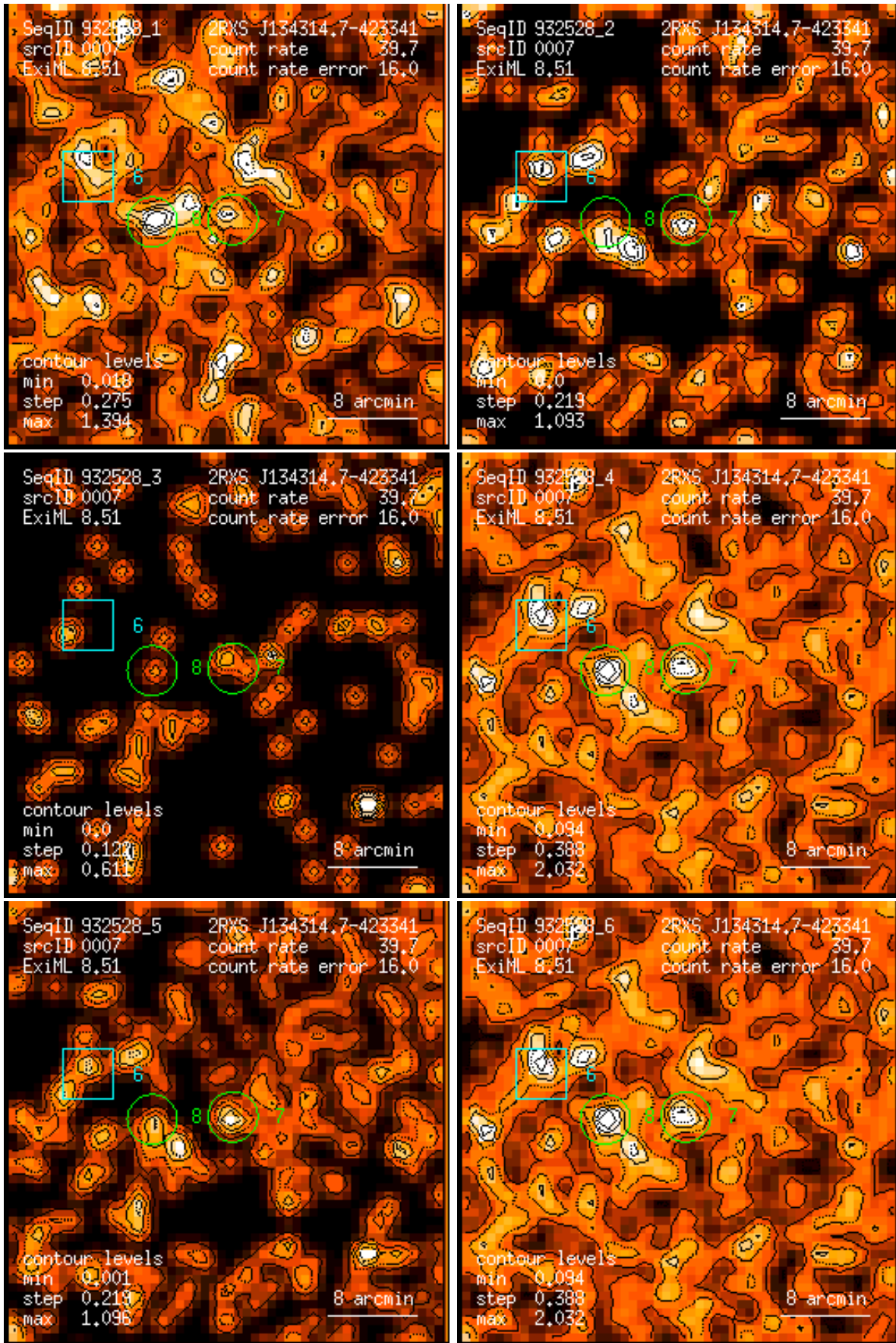
Figure 7: RASS 932528: detection 0007: band rate images, Gaussian filter: (1) PSPC channels 11 – 41, (2) 52 – 90, (3) 91 – 201, (4) 11 – 235, (5) 52 – 201, (6) 11 – 201. Broad band rates in counts/ks. Band rate contour levels in counts/ks/arcmin 2 .
