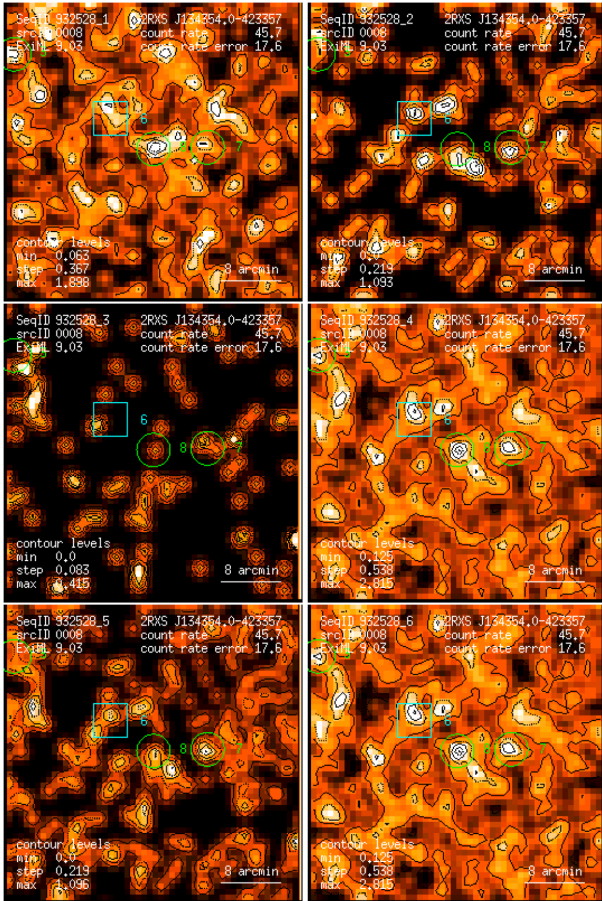
Figure 8: RASS 932528: detection 0008: band rate images, Gaussian filter: (1) PSPC channels 11 – 41, (2) 52 – 90, (3) 91 – 201, (4) 11 – 235, (5) 52 – 201, (6) 11 – 201. Broad band rates in counts/ks. Band rate contour levels in counts/ks/arcmin 2 .
