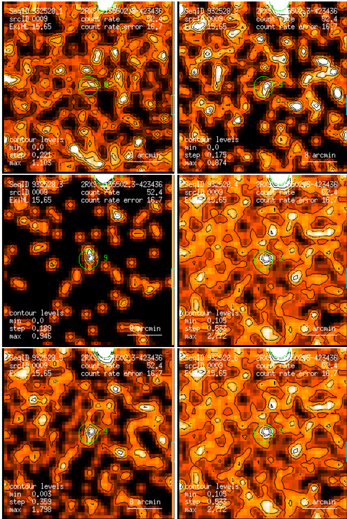
Figure 9: RASS 932528: detection 0009: band rate images, Gaussian filter: (1) PSPC channels 11 – 41, (2) 52 – 90, (3) 91 – 201, (4) 11 – 235, (5) 52 – 201, (6) 11 – 201. Broad band rates in counts/ks. Band rate contour levels in counts/ks/arcmin 2 .
