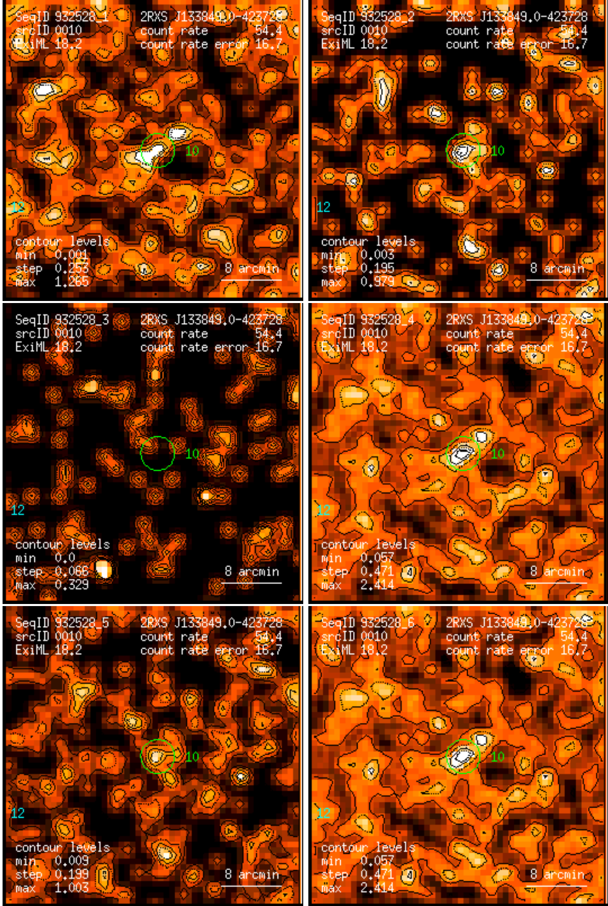
Figure 10: RASS 932528: detection 0010: band rate images, Gaussian filter: (1) PSPC channels 11 – 41, (2) 52 – 90, (3) 91 – 201, (4) 11 – 235, (5) 52 – 201, (6) 11 – 201. Broad band rates in counts/ks. Band rate contour levels in counts/ks/arcmin 2 .
