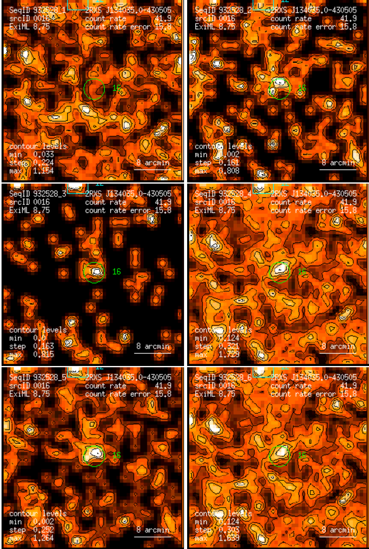
Figure 16: RASS 932528: detection 0016: band rate images, Gaussian filter: (1) PSPC channels 11 – 41, (2) 52 – 90, (3) 91 – 201, (4) 11 – 235, (5) 52 – 201, (6) 11 – 201. Broad band rates in counts/ks. Band rate contour levels in counts/ks/arcmin 2 .
