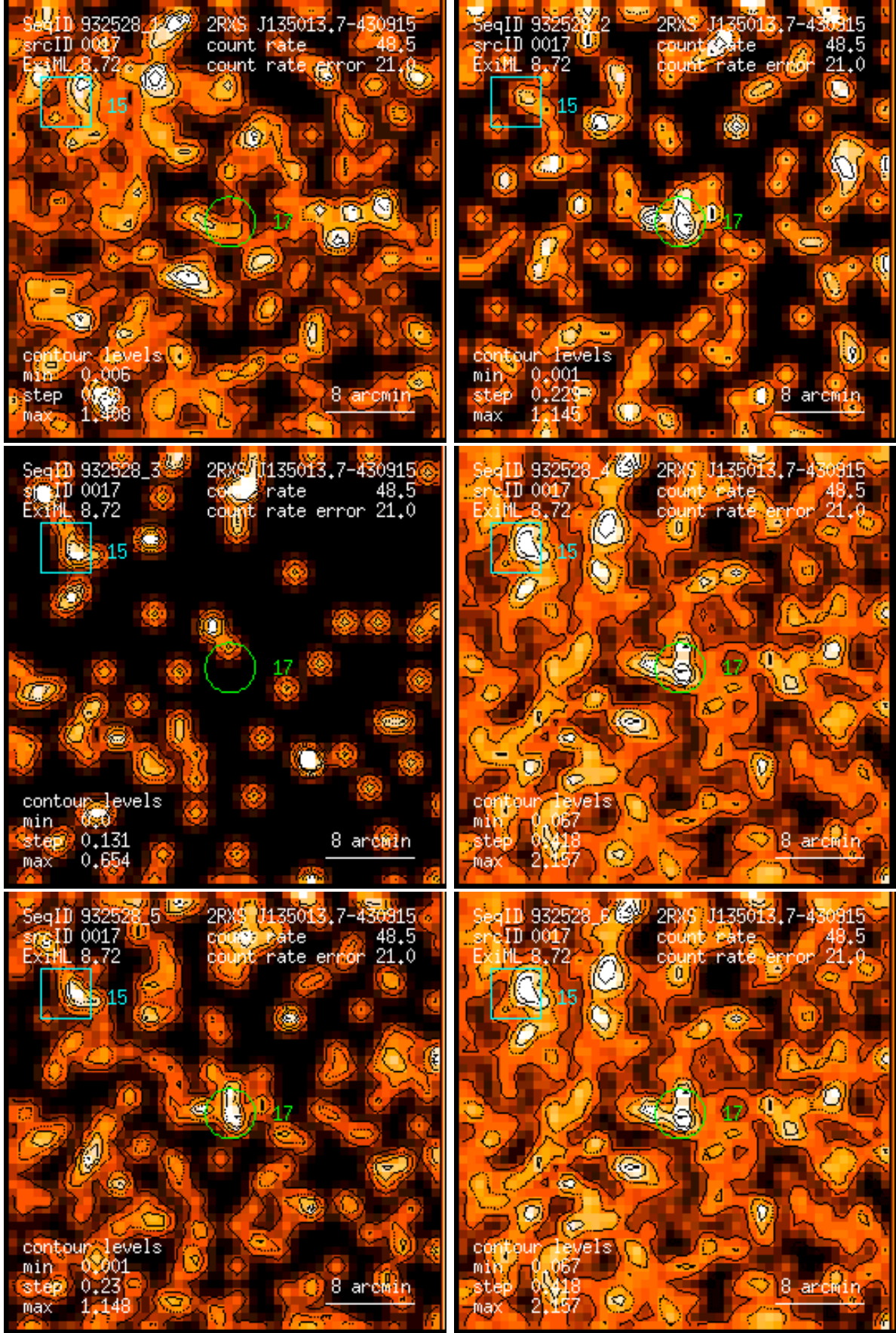
Figure 17: RASS 932528: detection 0017: band rate images, Gaussian filter: (1) PSPC channels 11 – 41, (2) 52 – 90, (3) 91 – 201, (4) 11 – 235, (5) 52 – 201, (6) 11 – 201. Broad band rates in counts/ks. Band rate contour levels in counts/ks/arcmin 2 .
