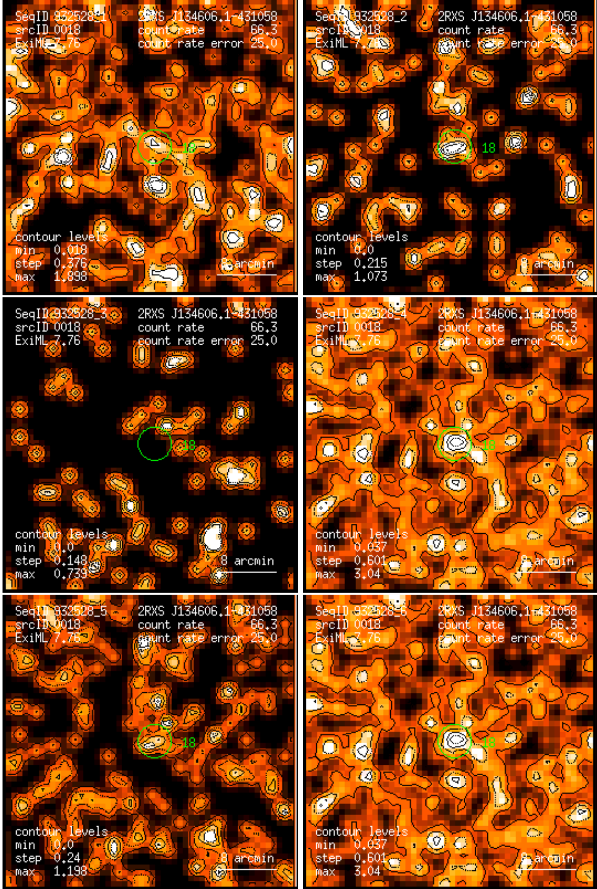
Figure 18: RASS 932528: detection 0018: band rate images, Gaussian filter: (1) PSPC channels 11 – 41, (2) 52 – 90, (3) 91 – 201, (4) 11 – 235, (5) 52 – 201, (6) 11 – 201. Broad band rates in counts/ks. Band rate contour levels in counts/ks/arcmin 2 .
