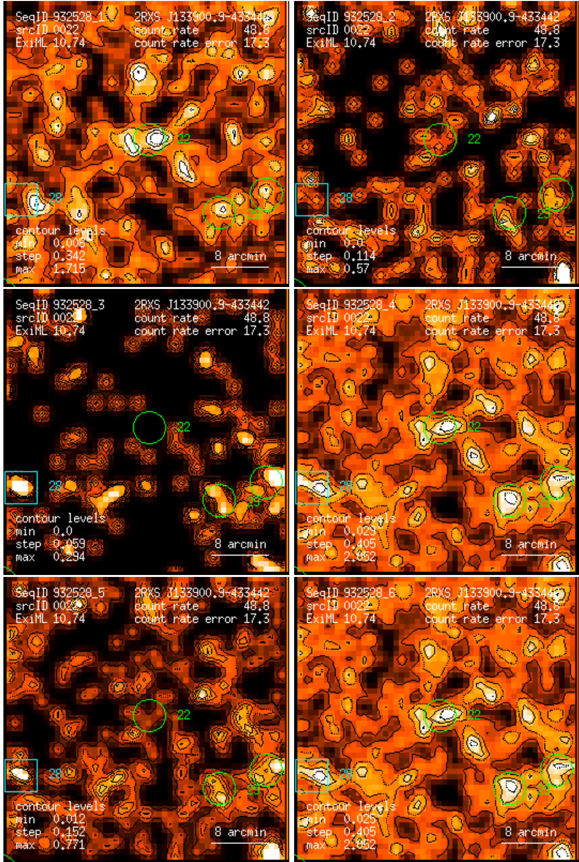
Figure 22: RASS 932528: detection 0022: band rate images, Gaussian filter: (1) PSPC channels 11 – 41, (2) 52 – 90, (3) 91 – 201, (4) 11 – 235, (5) 52 – 201, (6) 11 – 201. Broad band rates in counts/ks. Band rate contour levels in counts/ks/arcmin 2 .
