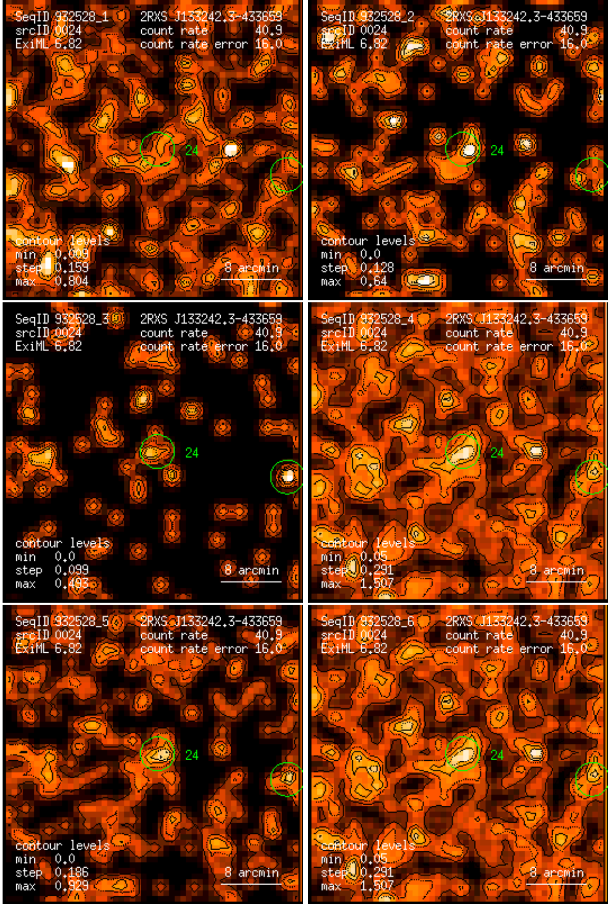
Figure 24: RASS 932528: detection 0024: band rate images, Gaussian filter: (1) PSPC channels 11 – 41, (2) 52 – 90, (3) 91 – 201, (4) 11 – 235, (5) 52 – 201, (6) 11 – 201. Broad band rates in counts/ks. Band rate contour levels in counts/ks/arcmin 2 .
