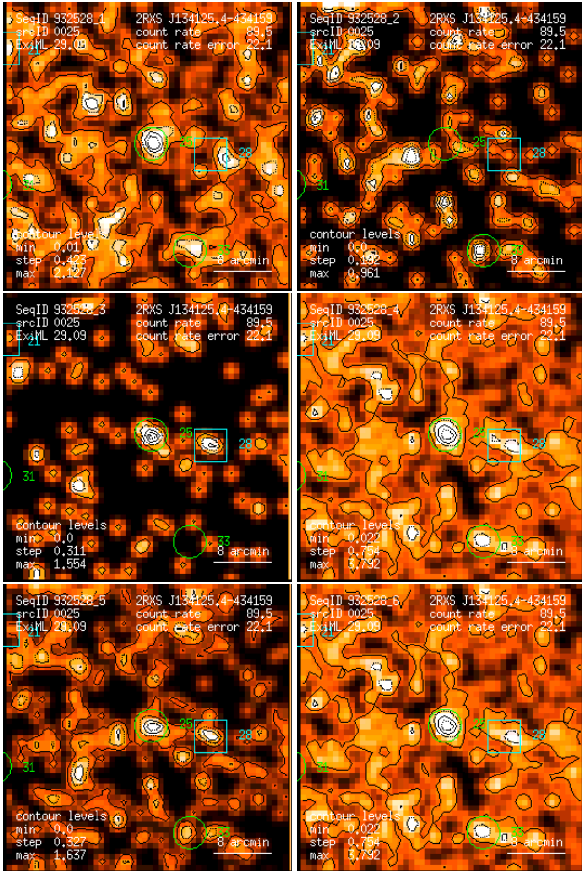
Figure 25: RASS 932528: detection 0025: band rate images, Gaussian filter: (1) PSPC channels 11 – 41, (2) 52 – 90, (3) 91 – 201, (4) 11 – 235, (5) 52 – 201, (6) 11 – 201. Broad band rates in counts/ks. Band rate contour levels in counts/ks/arcmin 2 .
