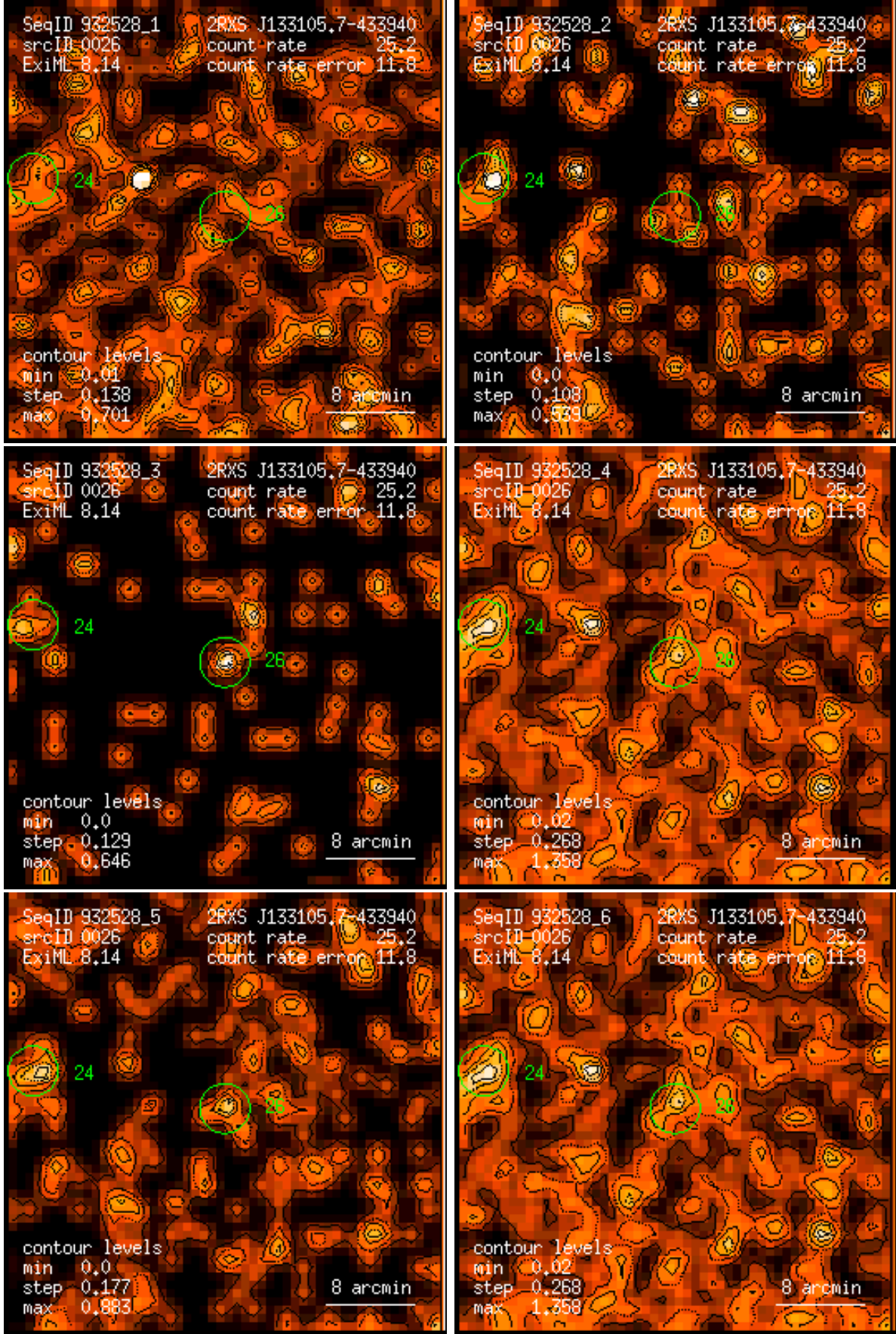
Figure 26: RASS 932528: detection 0026: band rate images, Gaussian filter: (1) PSPC channels 11 – 41, (2) 52 – 90, (3) 91 – 201, (4) 11 – 235, (5) 52 – 201, (6) 11 – 201. Broad band rates in counts/ks. Band rate contour levels in counts/ks/arcmin 2 .
