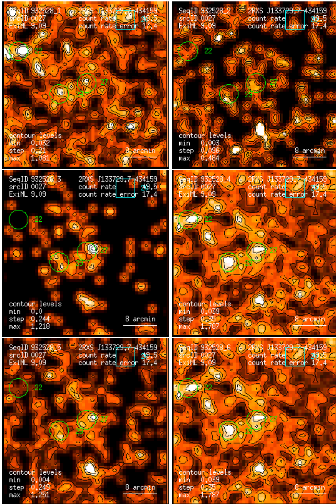
Figure 27: RASS 932528: detection 0027: band rate images, Gaussian filter: (1) PSPC channels 11 – 41, (2) 52 – 90, (3) 91 – 201, (4) 11 – 235, (5) 52 – 201, (6) 11 – 201. Broad band rates in counts/ks. Band rate contour levels in counts/ks/arcmin 2 .
