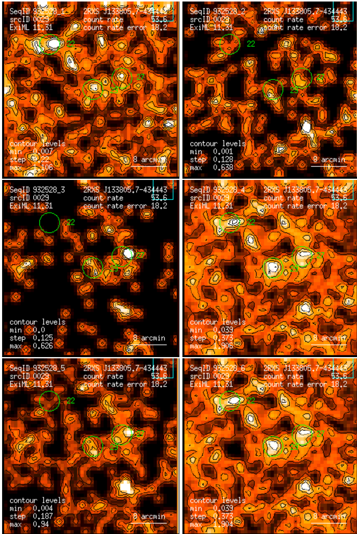
Figure 29: RASS 932528: detection 0029: band rate images, Gaussian filter: (1) PSPC channels 11 – 41, (2) 52 – 90, (3) 91 – 201, (4) 11 – 235, (5) 52 – 201, (6) 11 – 201. Broad band rates in counts/ks. Band rate contour levels in counts/ks/arcmin 2 .
