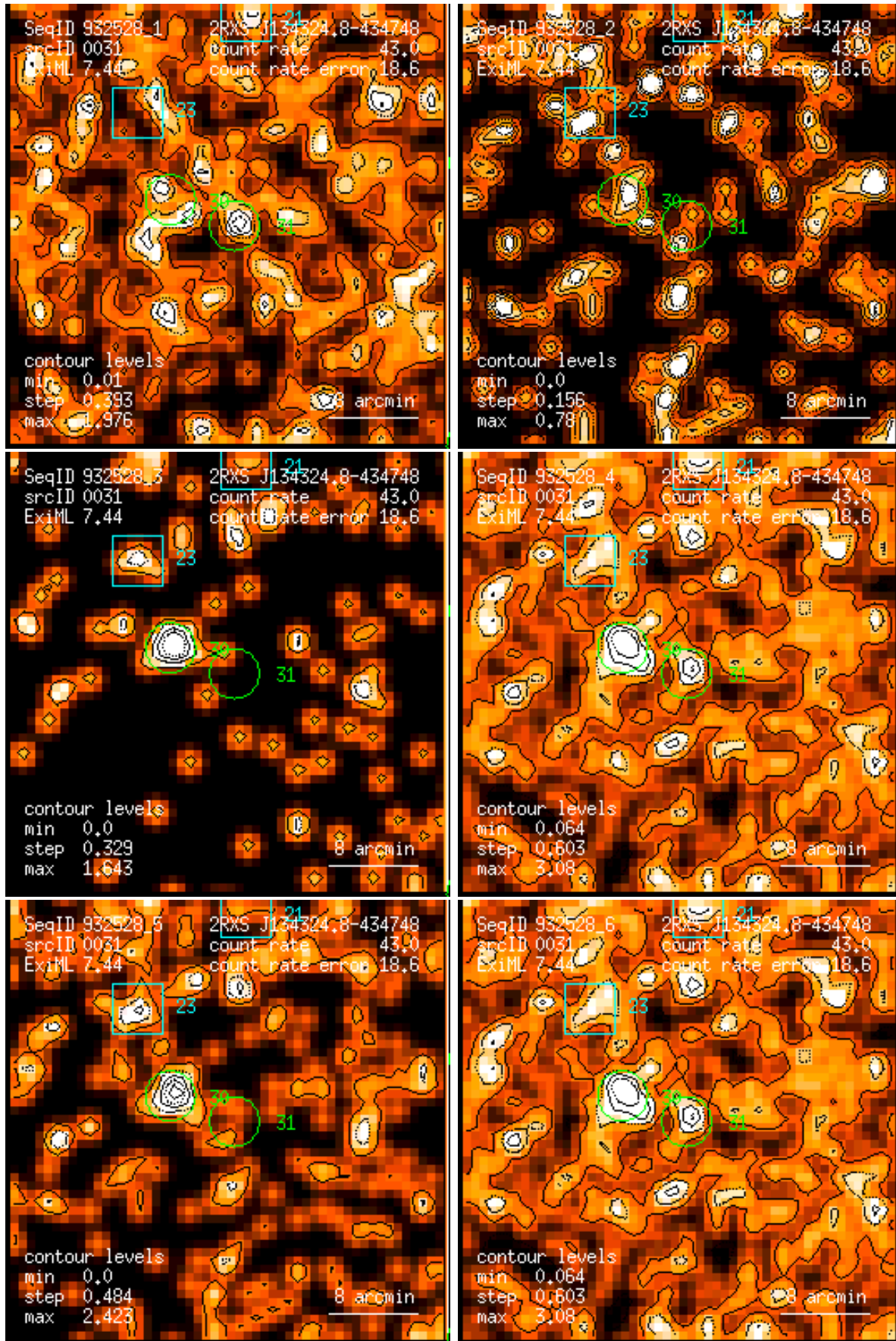
Figure 31: RASS 932528: detection 0031: band rate images, Gaussian filter: (1) PSPC channels 11 – 41, (2) 52 – 90, (3) 91 – 201, (4) 11 – 235, (5) 52 – 201, (6) 11 – 201. Broad band rates in counts/ks. Band rate contour levels in counts/ks/arcmin 2 .
