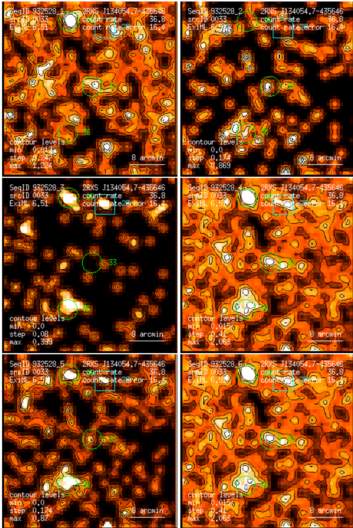
Figure 33: RASS 932528: detection 0033: band rate images, Gaussian filter: (1) PSPC channels 11 – 41, (2) 52 – 90, (3) 91 – 201, (4) 11 – 235, (5) 52 – 201, (6) 11 – 201. Broad band rates in counts/ks. Band rate contour levels in counts/ks/arcmin 2 .
