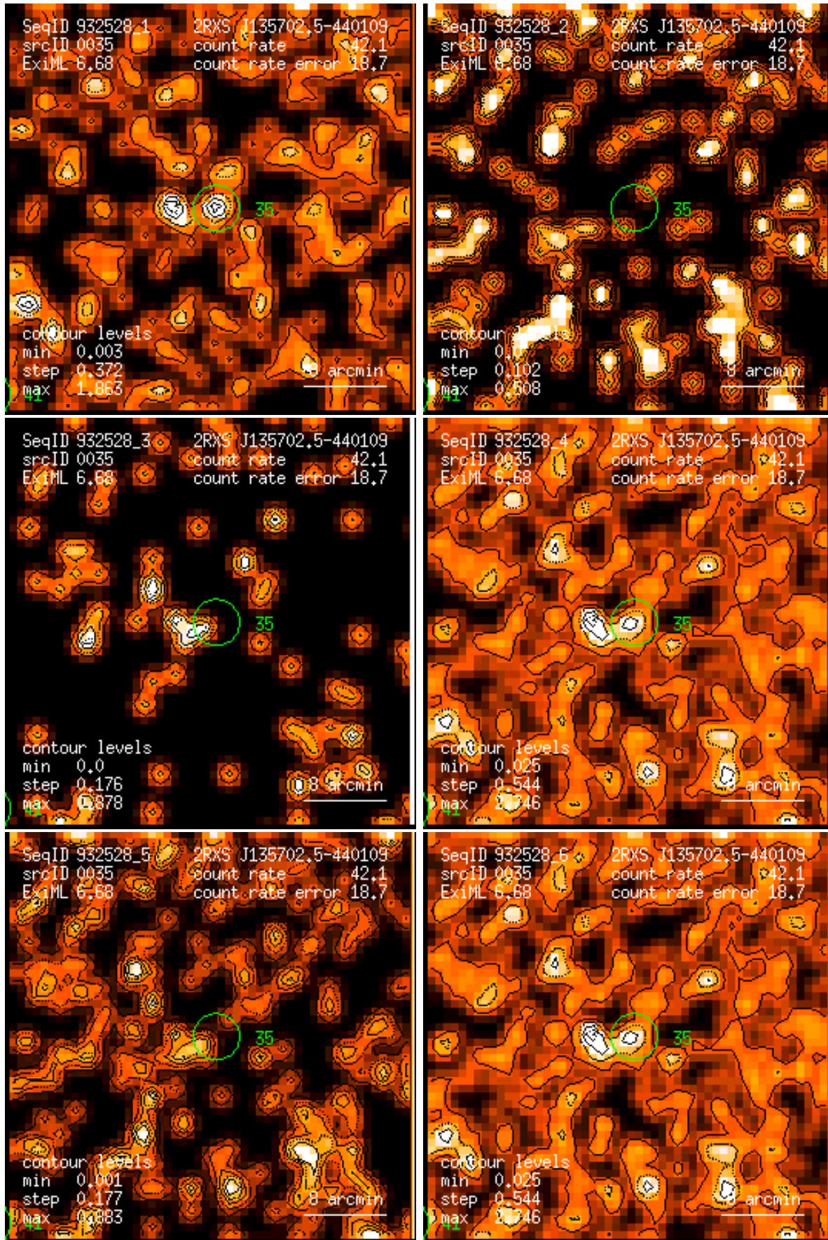
Figure 35: RASS 932528: detection 0035: band rate images, Gaussian filter: (1) PSPC channels 11 – 41, (2) 52 – 90, (3) 91 – 201, (4) 11 – 235, (5) 52 – 201, (6) 11 – 201. Broad band rates in counts/ks. Band rate contour levels in counts/ks/arcmin 2 .
