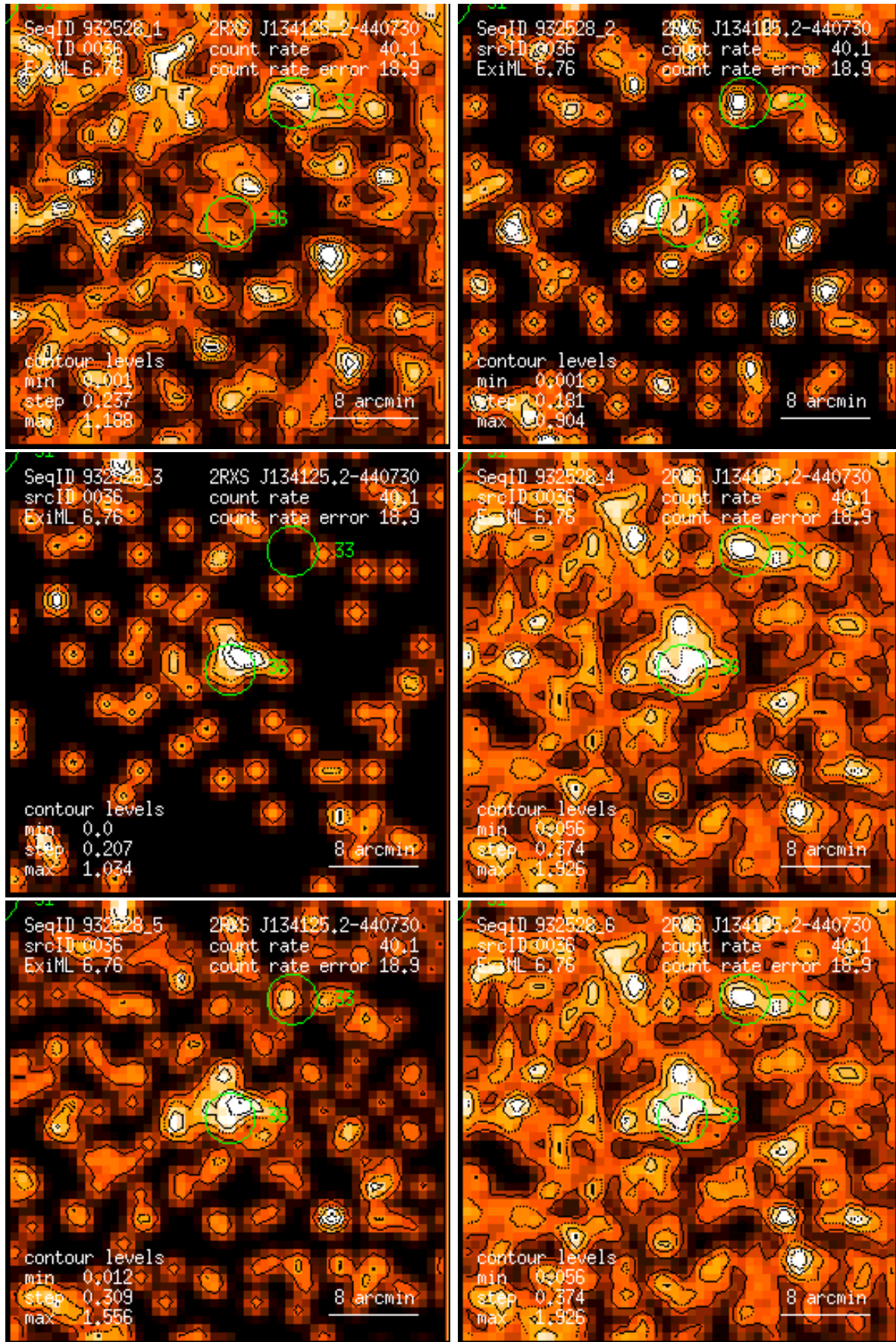
Figure 36: RASS 932528: detection 0036: band rate images, Gaussian filter: (1) PSPC channels 11 – 41, (2) 52 – 90, (3) 91 – 201, (4) 11 – 235, (5) 52 – 201, (6) 11 – 201. Broad band rates in counts/ks. Band rate contour levels in counts/ks/arcmin 2 .
