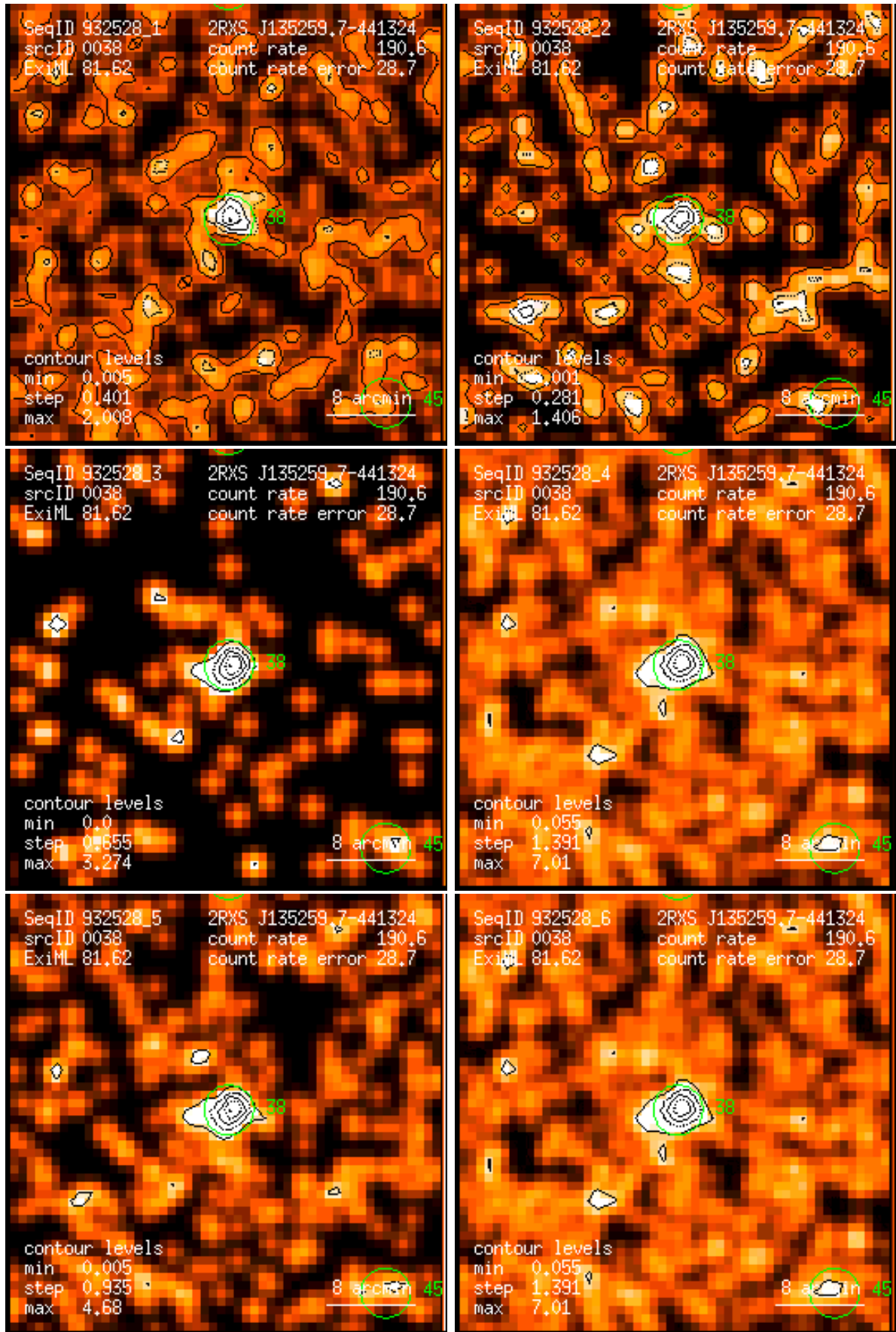
Figure 38: RASS 932528: detection 0038: band rate images, Gaussian filter: (1) PSPC channels 11 – 41, (2) 52 – 90, (3) 91 – 201, (4) 11 – 235, (5) 52 – 201, (6) 11 – 201. Broad band rates in counts/ks. Band rate contour levels in counts/ks/arcmin 2 .
