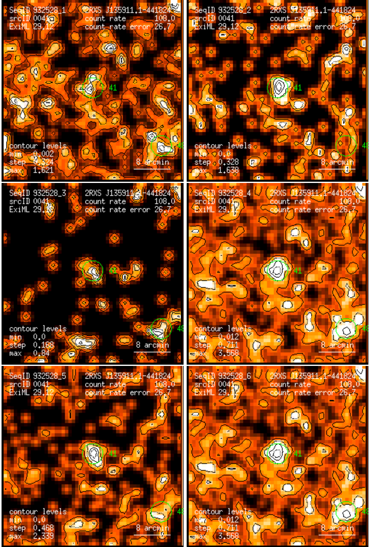
Figure 41: RASS 932528: detection 0041: band rate images, Gaussian filter: (1) PSPC channels 11 – 41, (2) 52 – 90, (3) 91 – 201, (4) 11 – 235, (5) 52 – 201, (6) 11 – 201. Broad band rates in counts/ks. Band rate contour levels in counts/ks/arcmin 2 .
