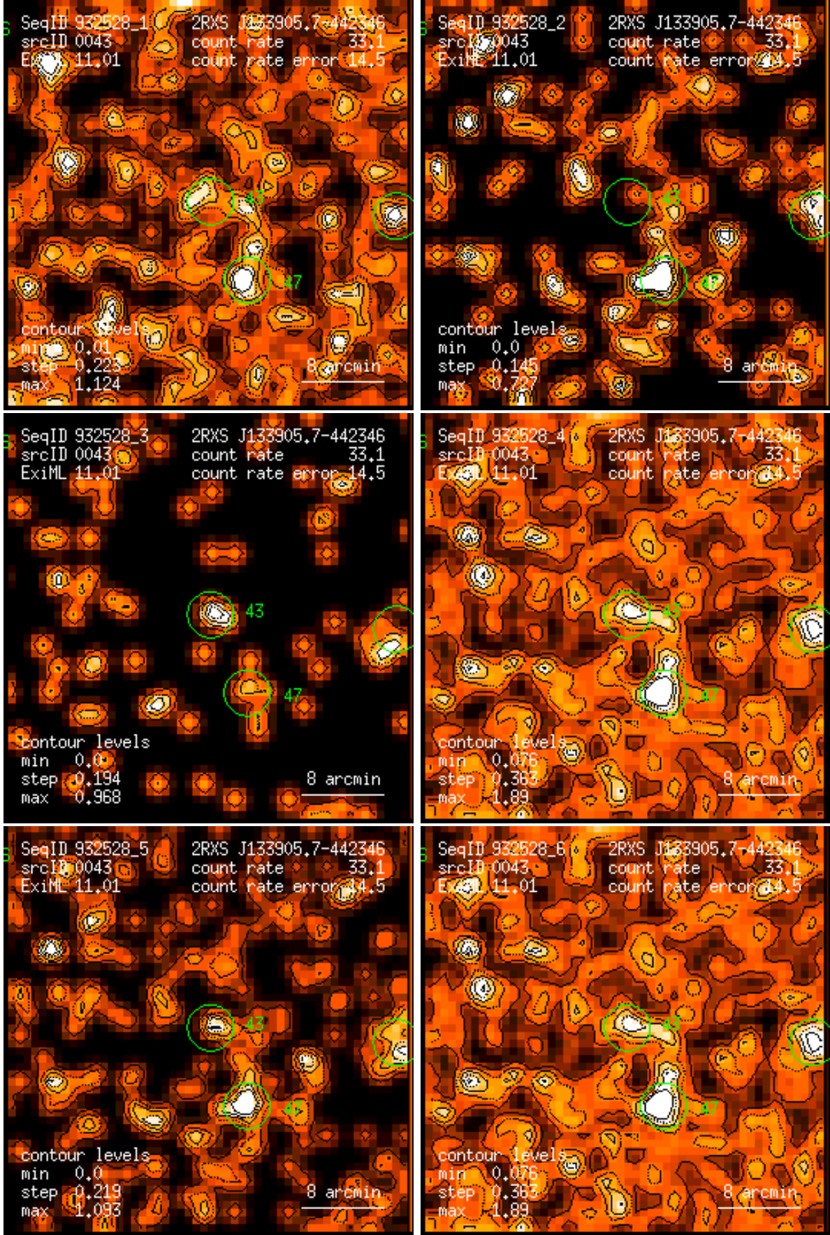
Figure 43: RASS 932528: detection 0043: band rate images, Gaussian filter: (1) PSPC channels 11 – 41, (2) 52 – 90, (3) 91 – 201, (4) 11 – 235, (5) 52 – 201, (6) 11 – 201. Broad band rates in counts/ks. Band rate contour levels in counts/ks/arcmin 2 .
