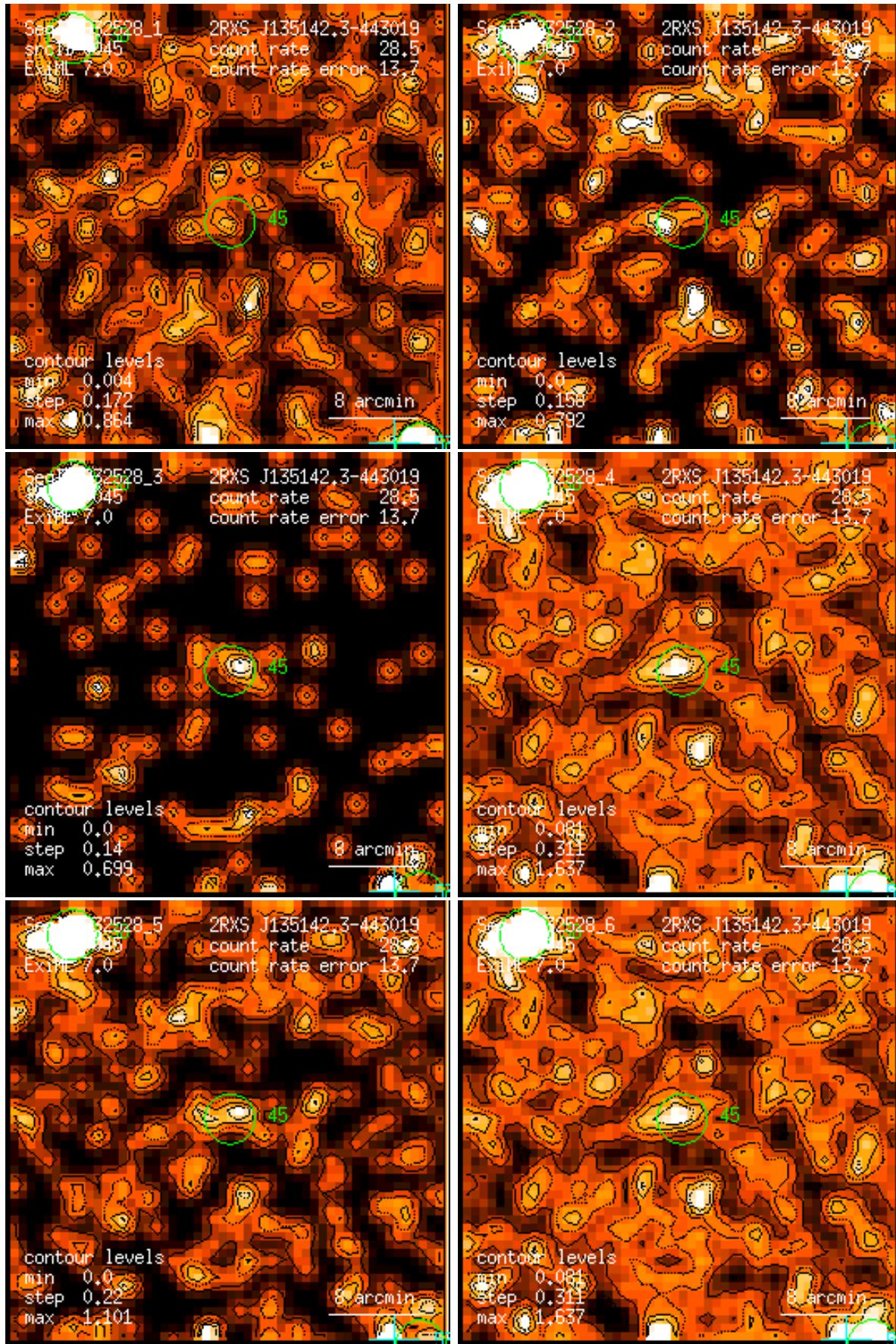
Figure 45: RASS 932528: detection 0045: band rate images, Gaussian filter: (1) PSPC channels 11 – 41, (2) 52 – 90, (3) 91 – 201, (4) 11 – 235, (5) 52 – 201, (6) 11 – 201. Broad band rates in counts/ks. Band rate contour levels in counts/ks/arcmin 2 .
