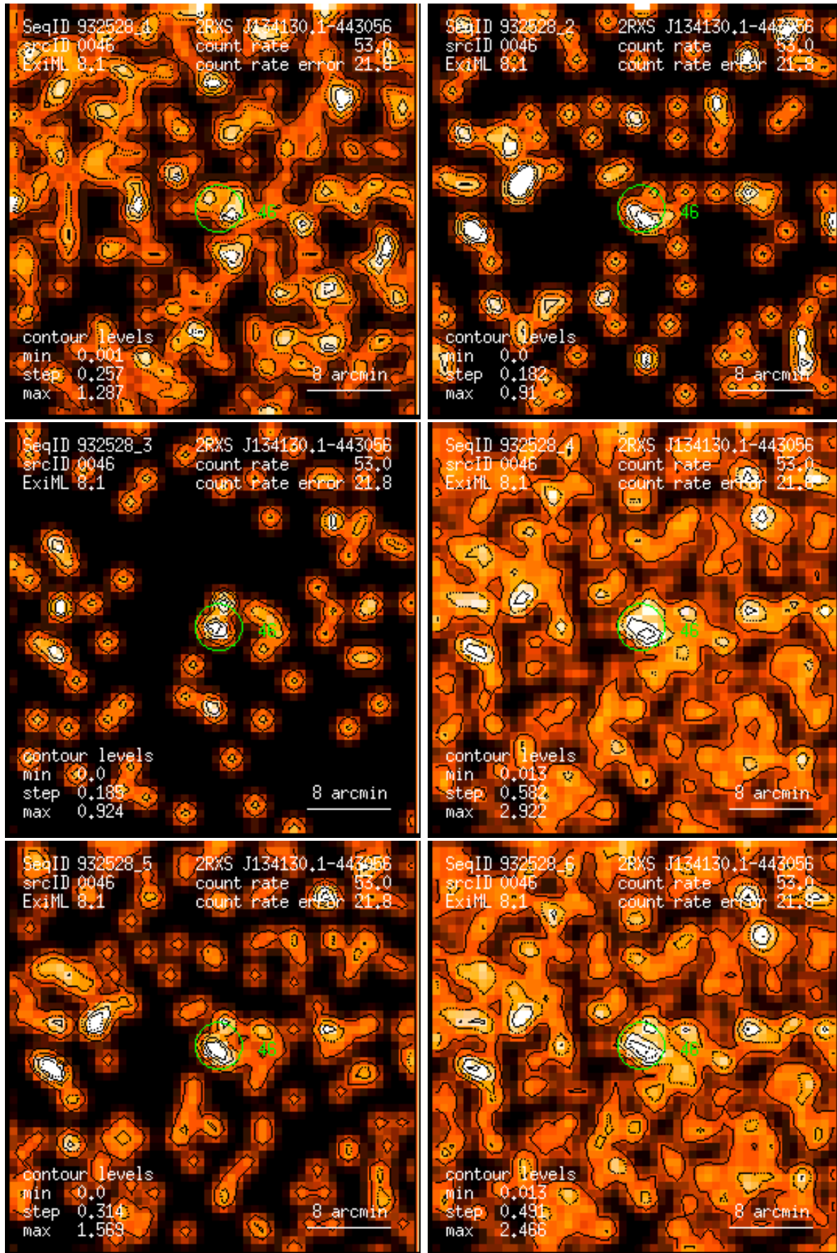
Figure 46: RASS 932528: detection 0046: band rate images, Gaussian filter: (1) PSPC channels 11 – 41, (2) 52 – 90, (3) 91 – 201, (4) 11 – 235, (5) 52 – 201, (6) 11 – 201. Broad band rates in counts/ks. Band rate contour levels in counts/ks/arcmin 2 .
