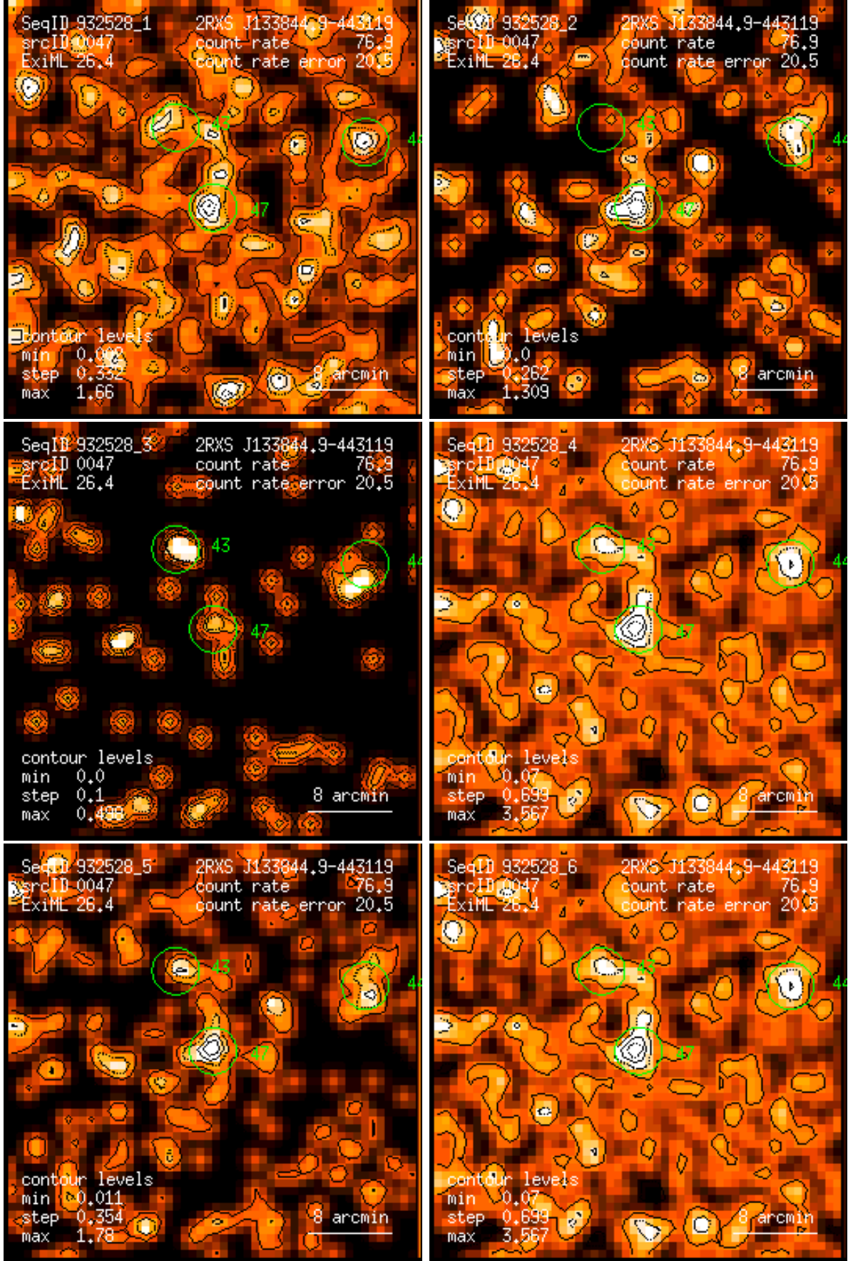
Figure 47: RASS 932528: detection 0047: band rate images, Gaussian filter: (1) PSPC channels 11 – 41, (2) 52 – 90, (3) 91 – 201, (4) 11 – 235, (5) 52 – 201, (6) 11 – 201. Broad band rates in counts/ks. Band rate contour levels in counts/ks/arcmin 2 .
