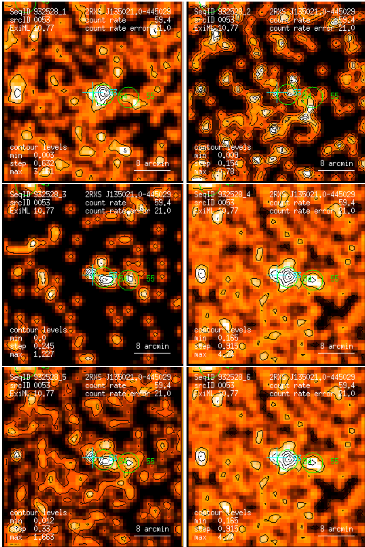
Figure 53: RASS 932528: detection 0053: band rate images, Gaussian filter: (1) PSPC channels 11 – 41, (2) 52 – 90, (3) 91 – 201, (4) 11 – 235, (5) 52 – 201, (6) 11 – 201. Broad band rates in counts/ks. Band rate contour levels in counts/ks/arcmin 2 .
