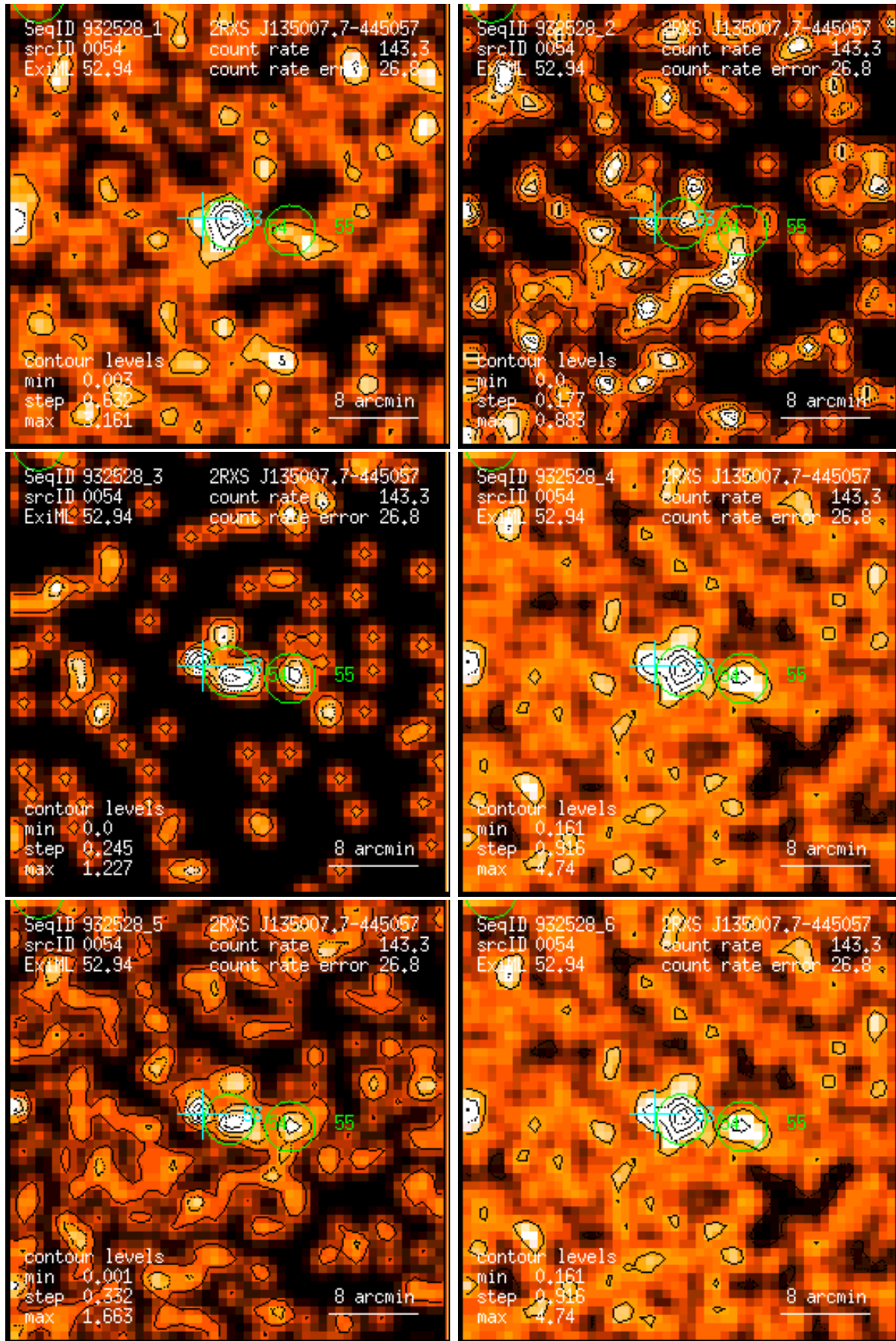
Figure 54: RASS 932528: detection 0054: band rate images, Gaussian filter: (1) PSPC channels 11 – 41, (2) 52 – 90, (3) 91 – 201, (4) 11 – 235, (5) 52 – 201, (6) 11 – 201. Broad band rates in counts/ks. Band rate contour levels in counts/ks/arcmin 2 .
