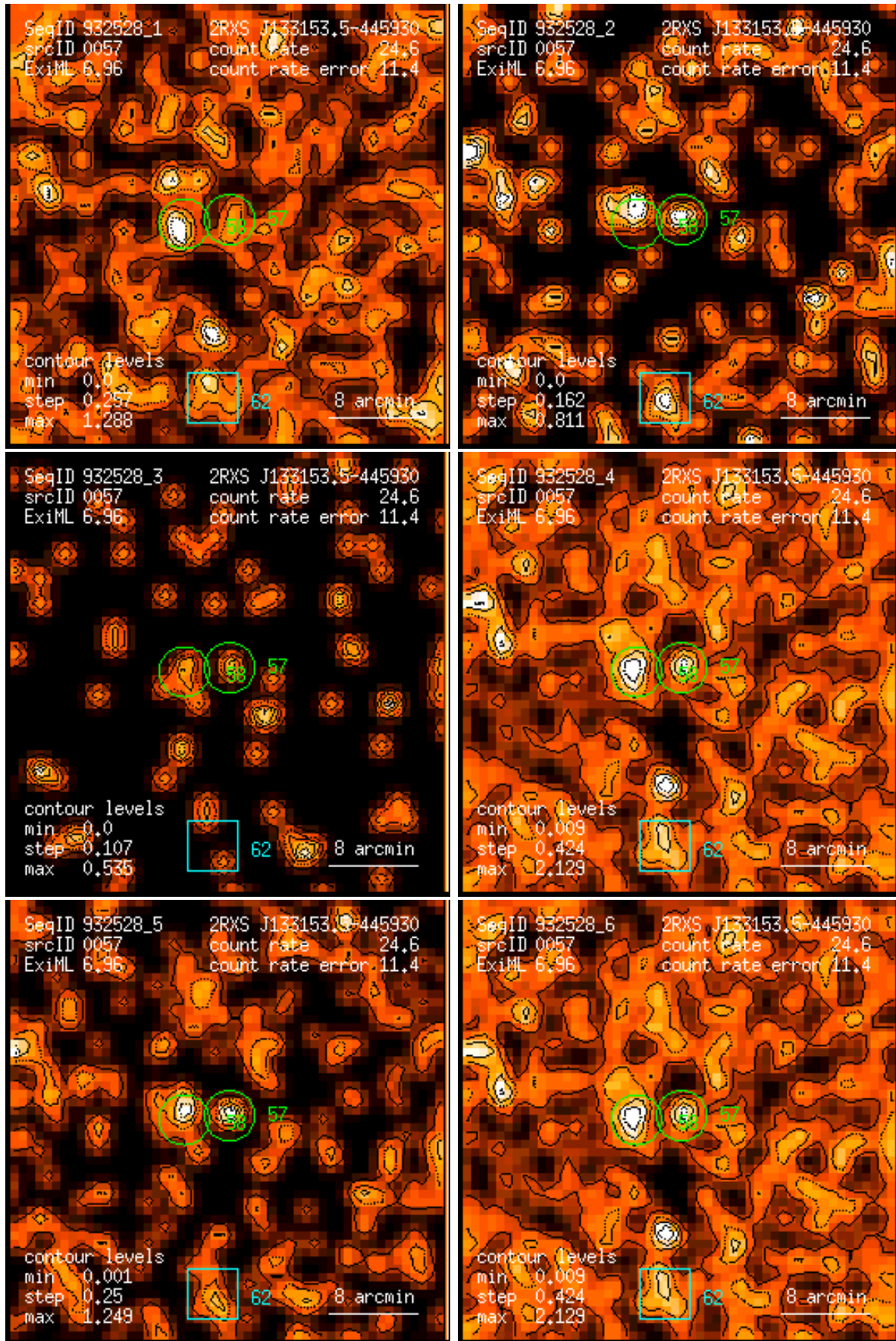
Figure 57: RASS 932528: detection 0057: band rate images, Gaussian filter: (1) PSPC channels 11 – 41, (2) 52 – 90, (3) 91 – 201, (4) 11 – 235, (5) 52 – 201, (6) 11 – 201. Broad band rates in counts/ks. Band rate contour levels in counts/ks/arcmin 2 .
