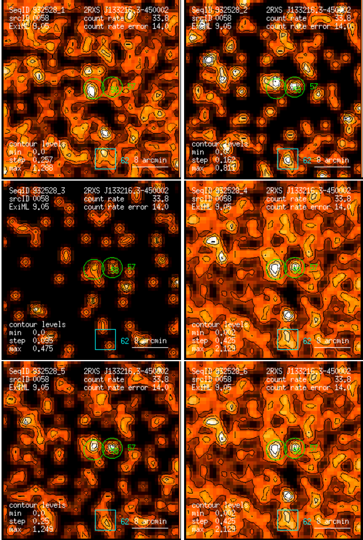
Figure 58: RASS 932528: detection 0058: band rate images, Gaussian filter: (1) PSPC channels 11 – 41, (2) 52 – 90, (3) 91 – 201, (4) 11 – 235, (5) 52 – 201, (6) 11 – 201. Broad band rates in counts/ks. Band rate contour levels in counts/ks/arcmin 2 .
