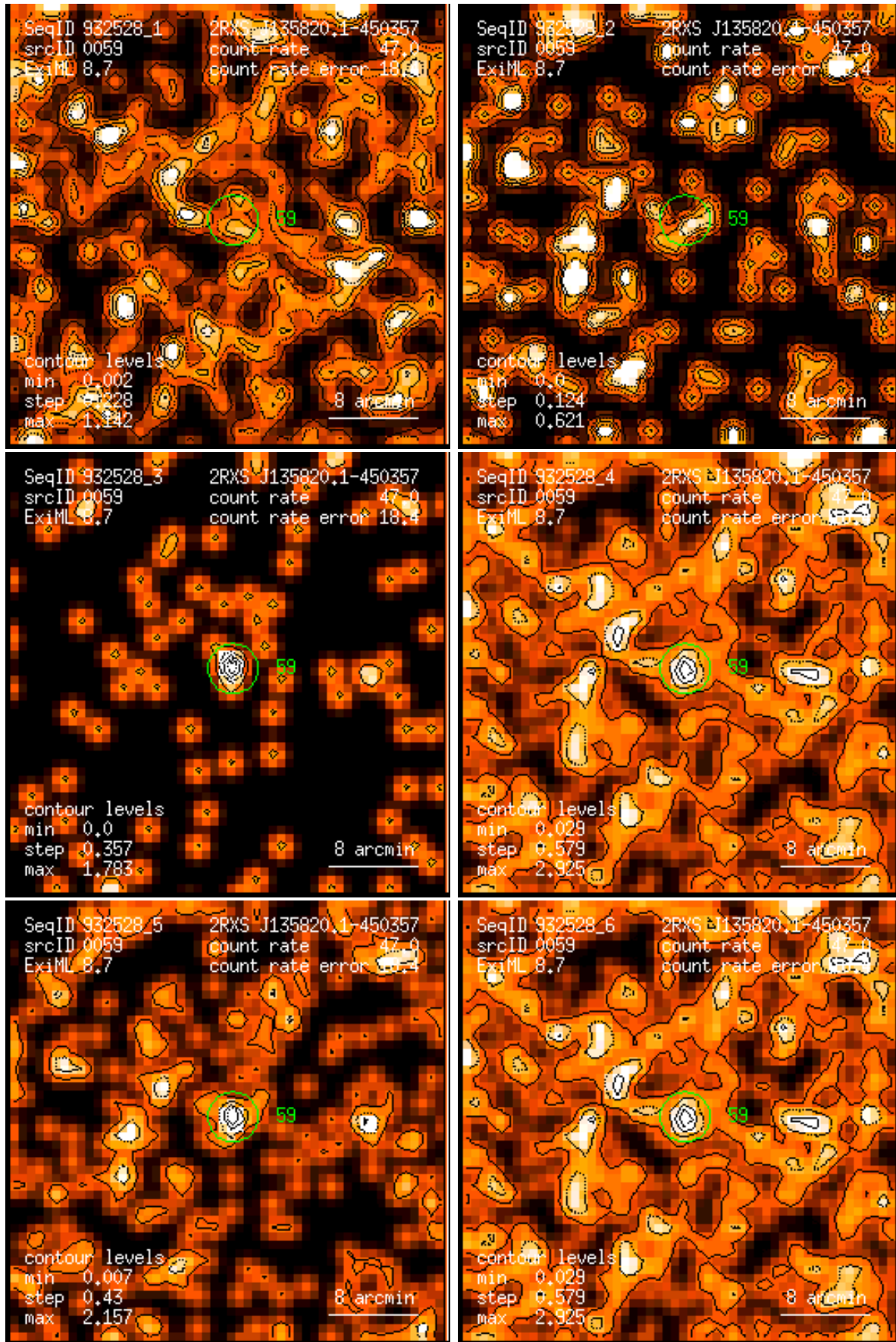
Figure 59: RASS 932528: detection 0059: band rate images, Gaussian filter: (1) PSPC channels 11 – 41, (2) 52 – 90, (3) 91 – 201, (4) 11 – 235, (5) 52 – 201, (6) 11 – 201. Broad band rates in counts/ks. Band rate contour levels in counts/ks/arcmin 2 .
