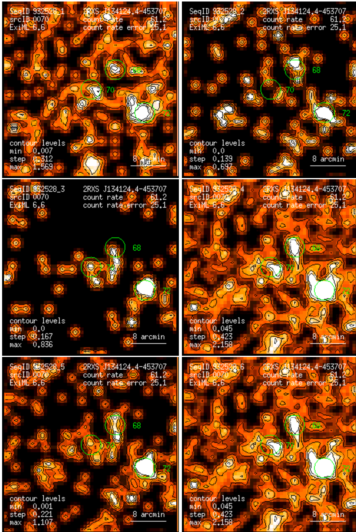
Figure 70: RASS 932528: detection 0070: band rate images, Gaussian filter: (1) PSPC channels 11 – 41, (2) 52 – 90, (3) 91 – 201, (4) 11 – 235, (5) 52 – 201, (6) 11 – 201. Broad band rates in counts/ks. Band rate contour levels in counts/ks/arcmin 2 .
