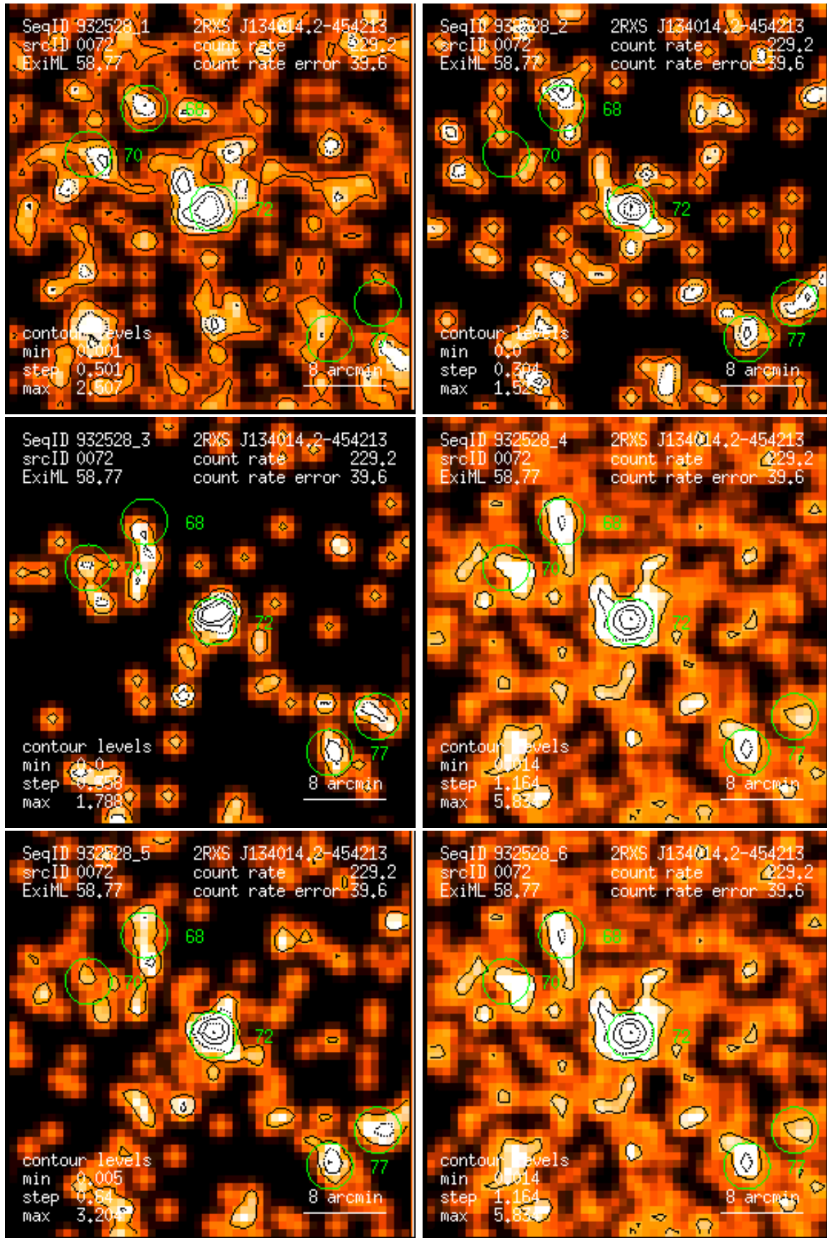
Figure 72: RASS 932528: detection 0072: band rate images, Gaussian filter: (1) PSPC channels 11 – 41, (2) 52 – 90, (3) 91 – 201, (4) 11 – 235, (5) 52 – 201, (6) 11 – 201. Broad band rates in counts/ks. Band rate contour levels in counts/ks/arcmin 2 .
