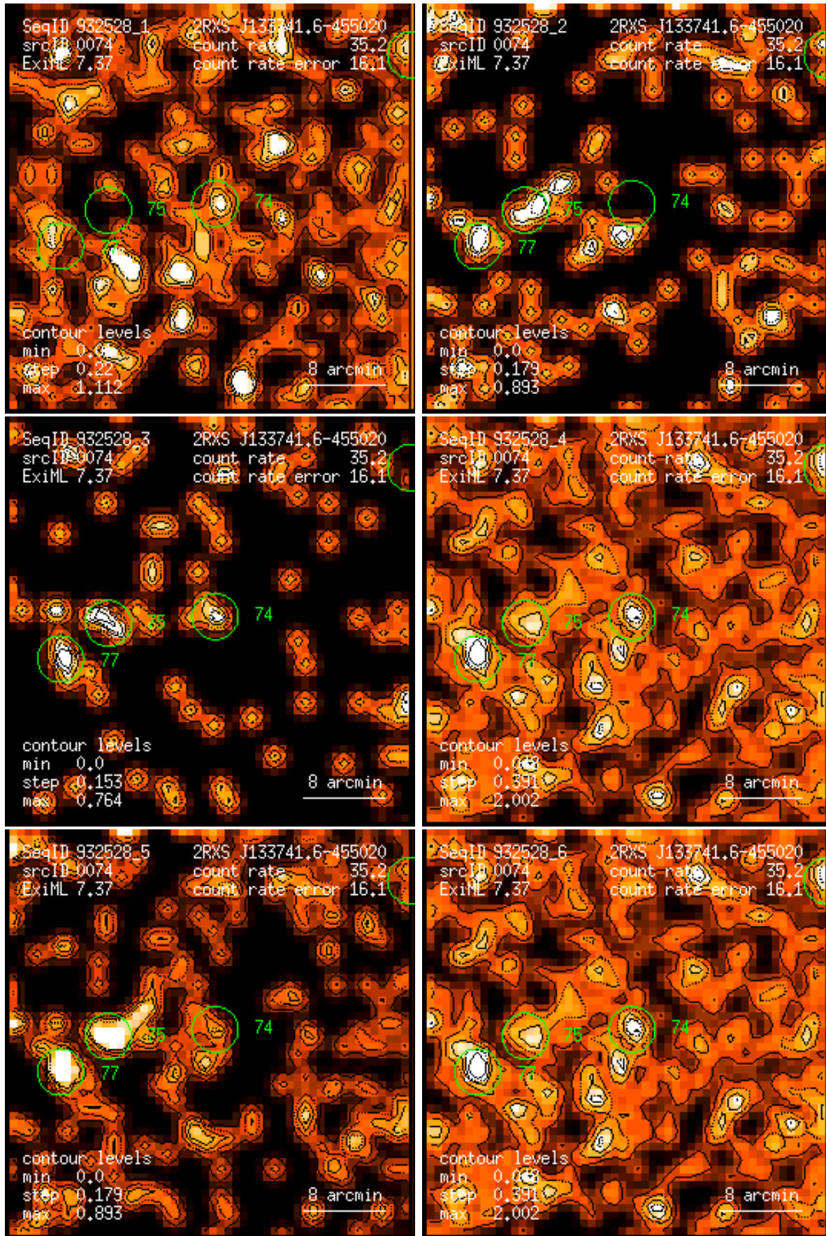
Figure 74: RASS 932528: detection 0074: band rate images, Gaussian filter: (1) PSPC channels 11 – 41, (2) 52 – 90, (3) 91 – 201, (4) 11 – 235, (5) 52 – 201, (6) 11 – 201. Broad band rates in counts/ks. Band rate contour levels in counts/ks/arcmin 2 .
