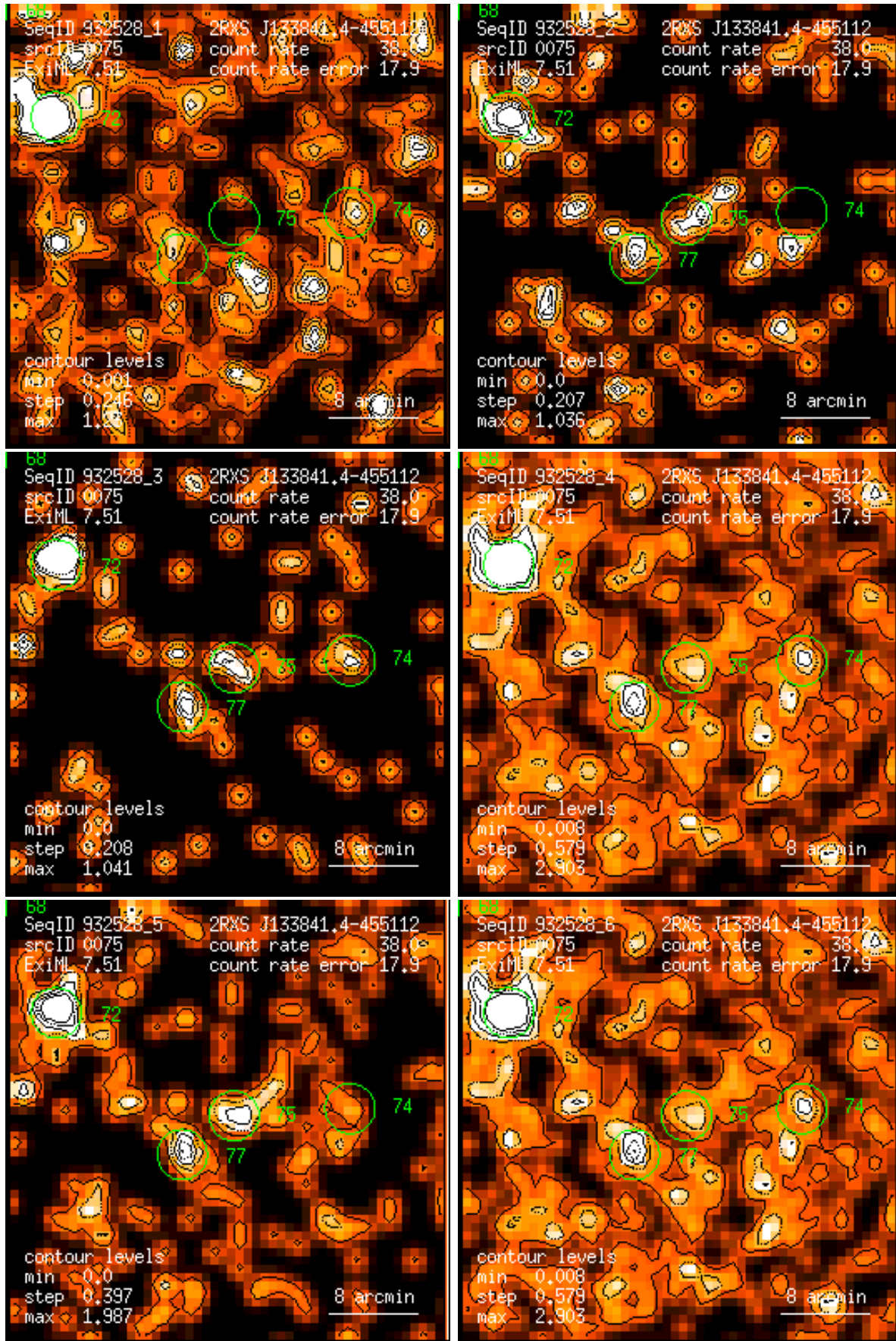
Figure 75: RASS 932528: detection 0075: band rate images, Gaussian filter: (1) PSPC channels 11 – 41, (2) 52 – 90, (3) 91 – 201, (4) 11 – 235, (5) 52 – 201, (6) 11 – 201. Broad band rates in counts/ks. Band rate contour levels in counts/ks/arcmin 2 .
